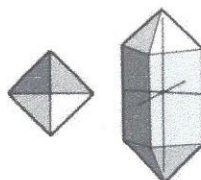
Tetragonal
