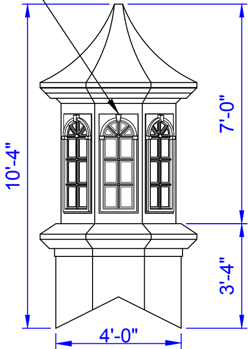
Elevation View
