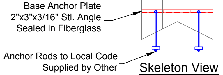
Mounting Detail
