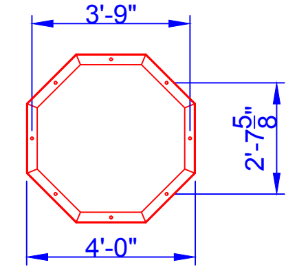
Mounting Detail
