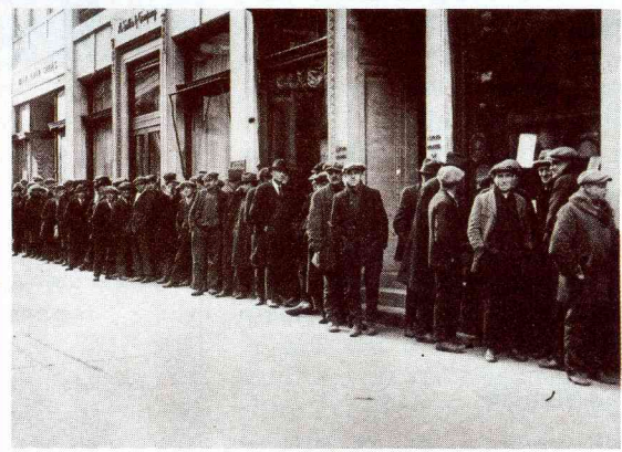
The Great Depression continues.
