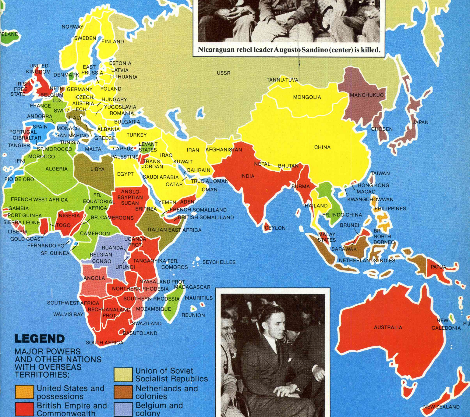
Bruno Hauptmann is arrested for kidnapping the Lindbergh baby.
