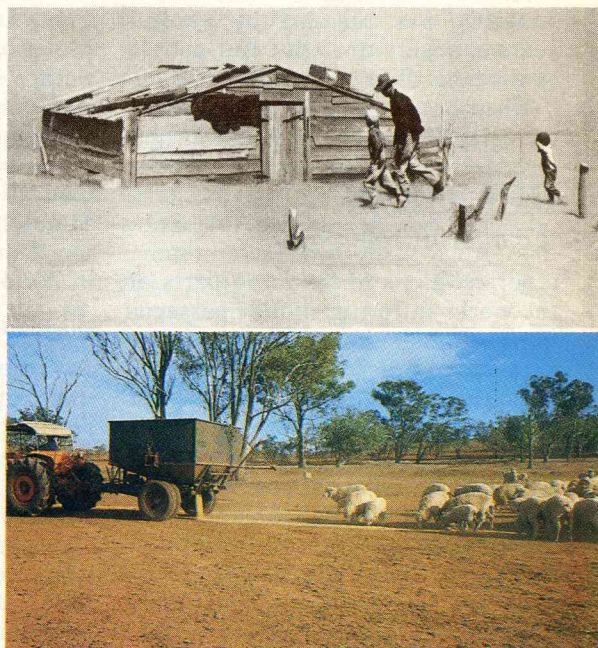
The devastation of the U.S. dust bowl in the 1930s (top) was repeated in recent decades in Australia.
