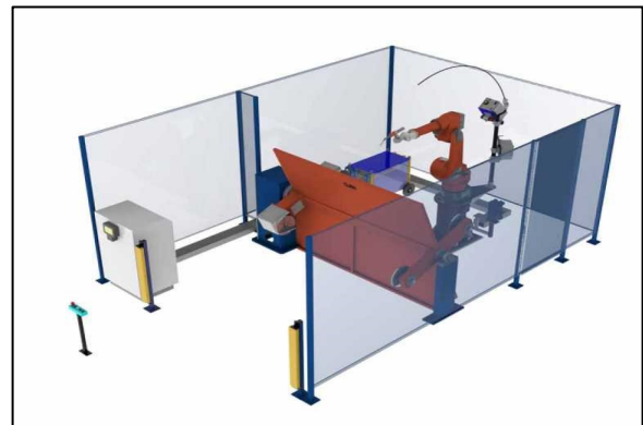
Weld Cell with Automatic Rotating Part Positioner
