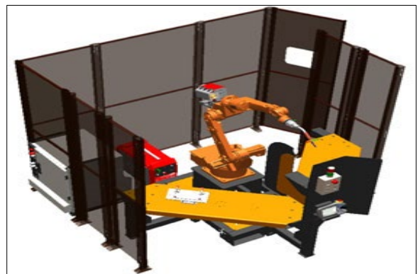
Small Part Weld Cell with Work Piece Tables
