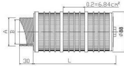
Lateral Ø88: LAT88
