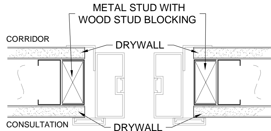
B JAMB DETAIL OF ROUGH OPENING SCALE: NTS
