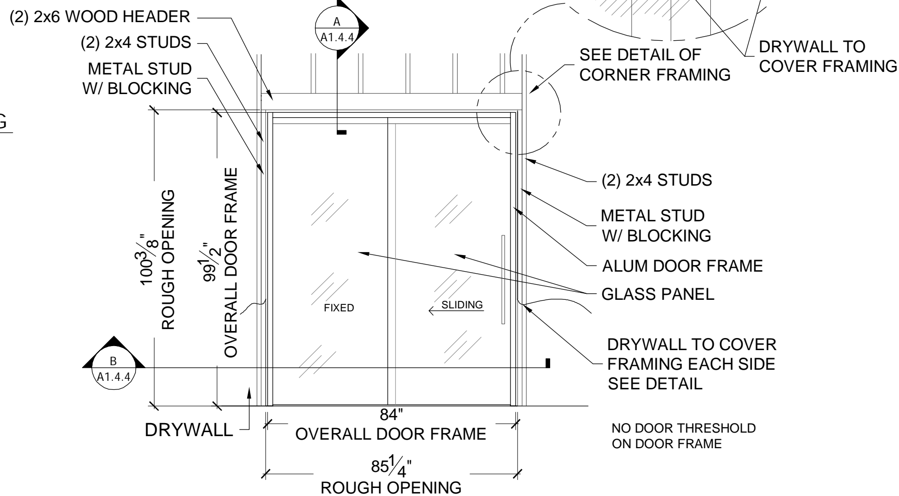
1 SLIDING DOOR ELEVATION SCALE: 3/8" = 1'-0"
