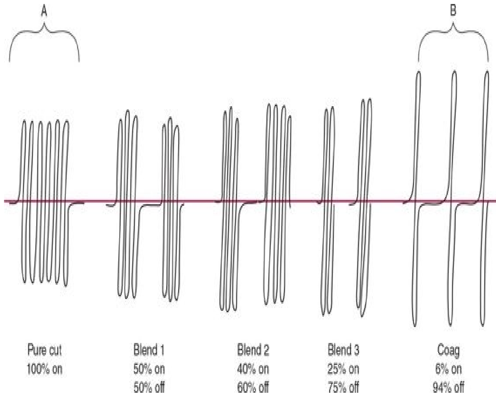
▲ Figure 7–3. Electrosurgical waveforms. A. Cutting current. B. Coagulation current.
