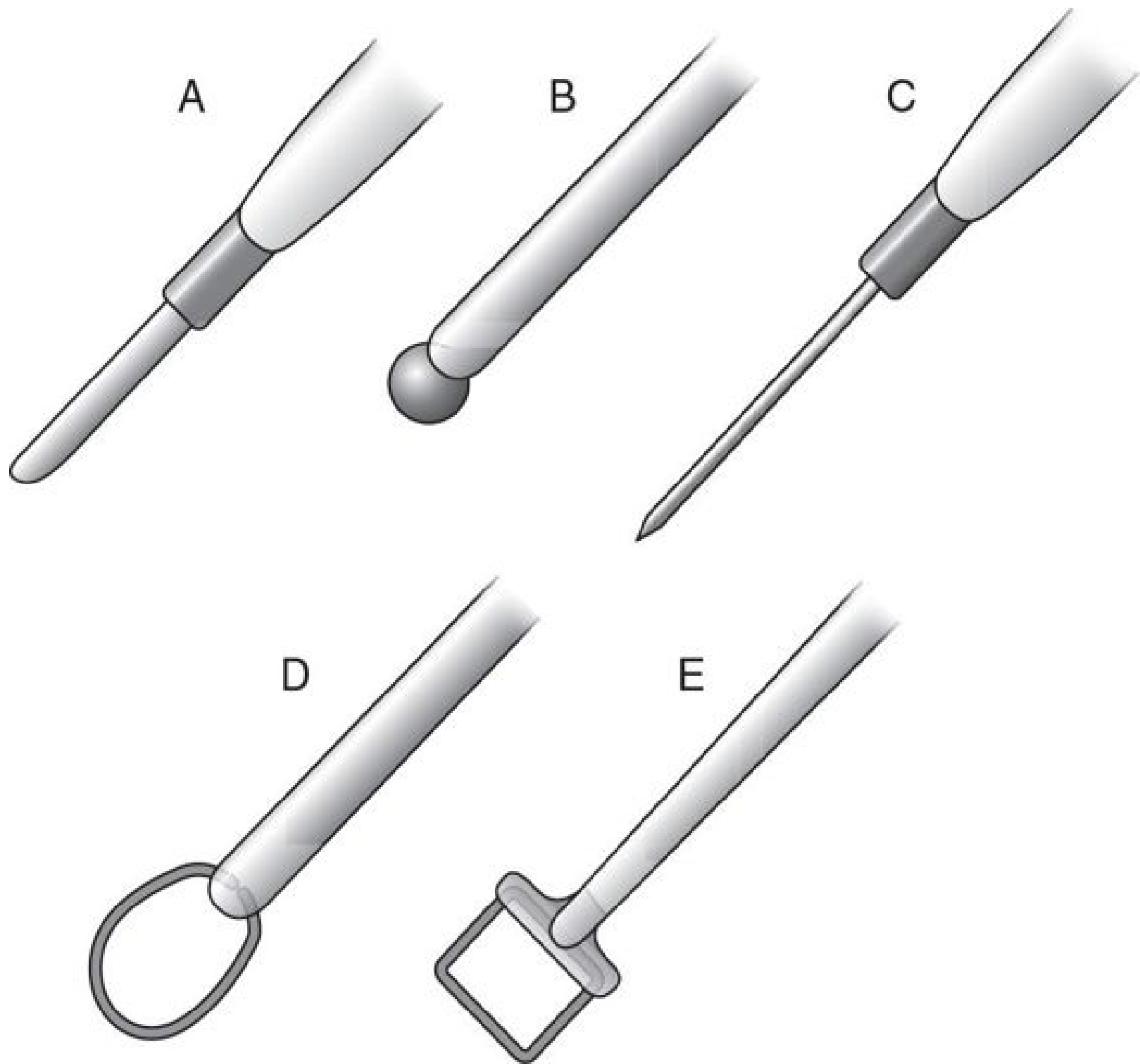
▲ Figure 7-4. A. Knife electrode. B. Ball electrode. C. Needle electrode. D. Loop electrode. E. Wire electrode.
