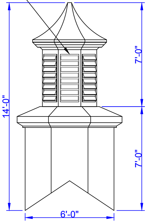
Elevation View
