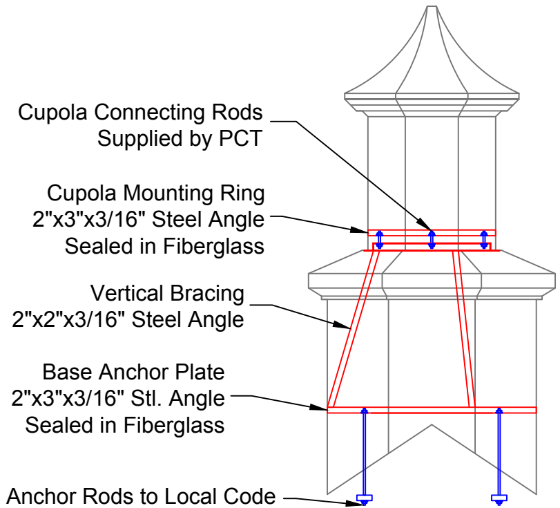
Skeleton View
