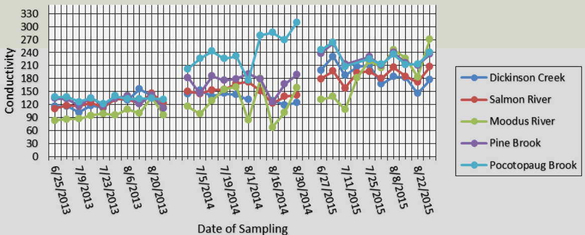
Salmon River Watershed (Lower)-uS/cm
