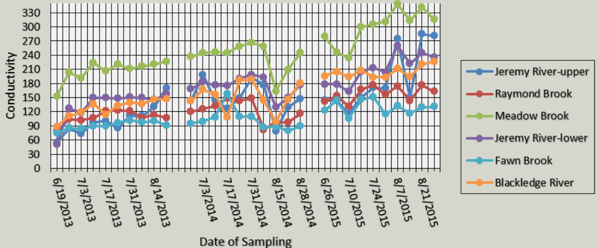
Salmon River Watershed (Upper)-uS/cm
