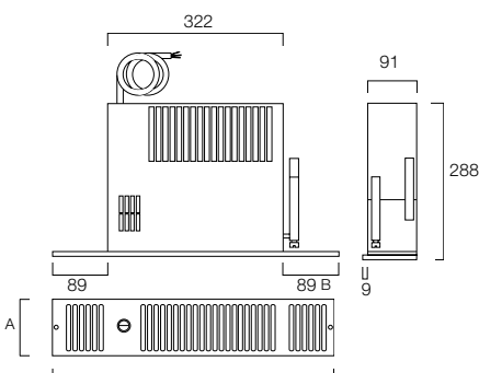
Plinth Hydronic
