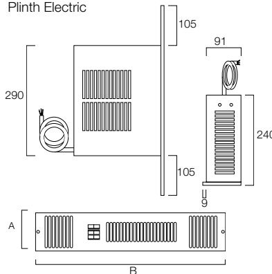
Plinth Electric
