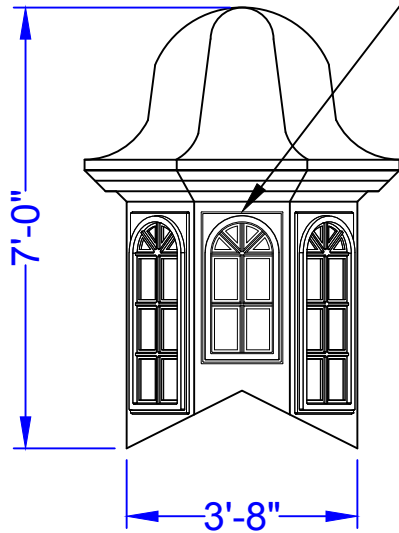
Elevation View
