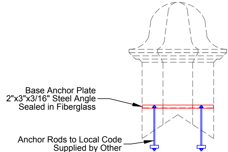
Skeleton View
