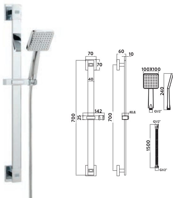
Lunar Slide Rail Kit
