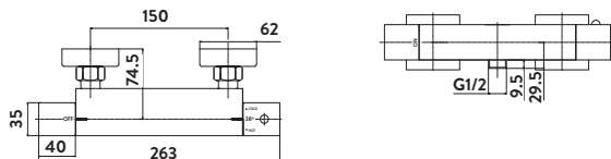
Square Exposed Valve
