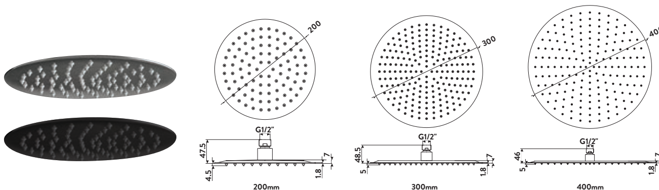
Black Round Shower Heads
