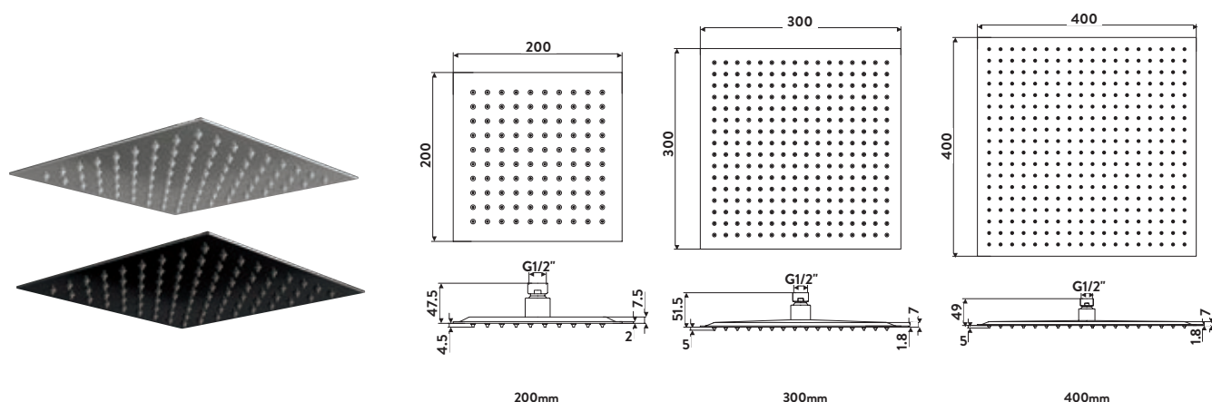
Chrome Square Shower Head
