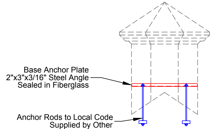
Skeleton View
