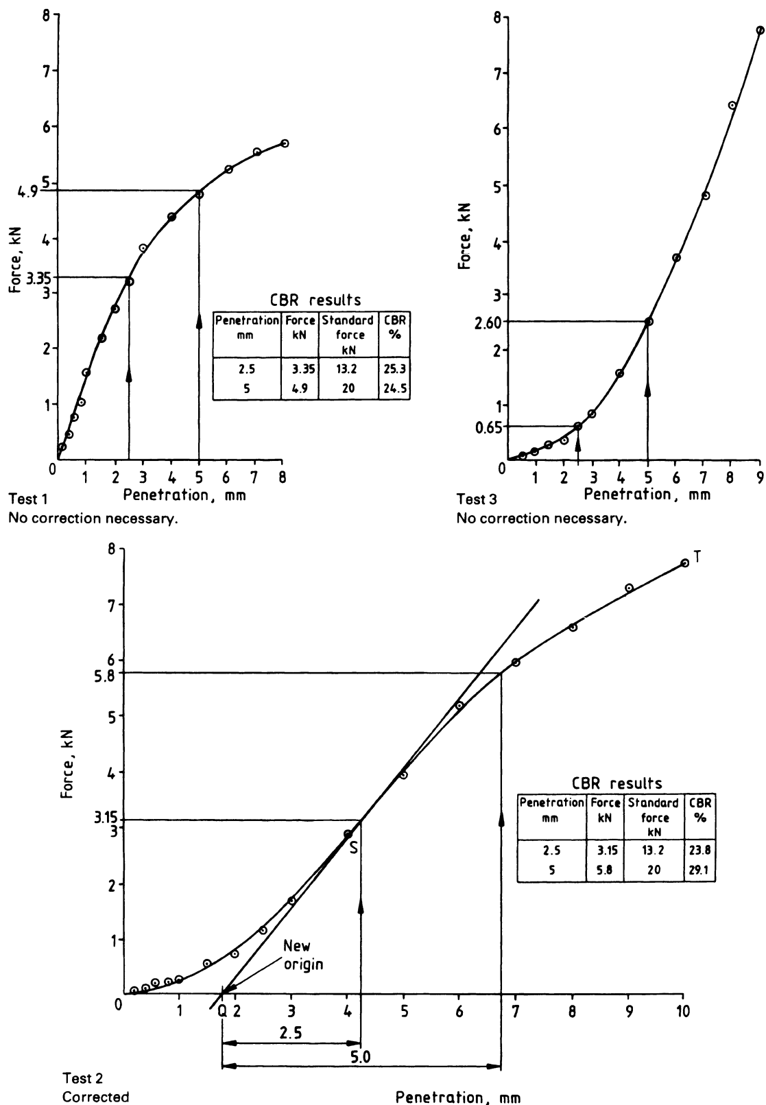
Figure 14 — Typical CBR test results curves
