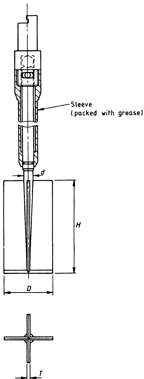
Figure 17 — Typical borehole vane and rod mounting
