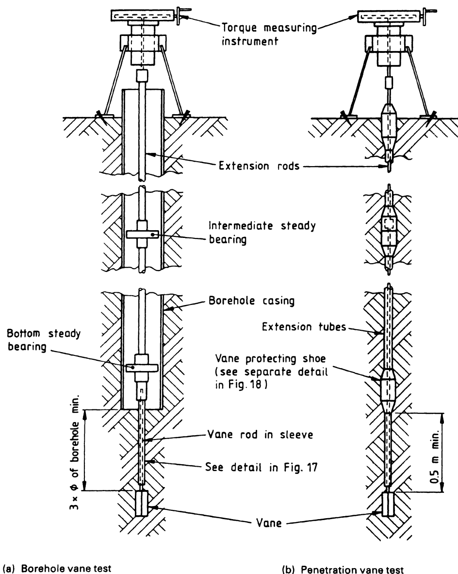
Figure 16 — Typical arrangements for in-situ vane test apparatus
