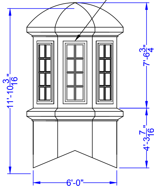
Elevation View
