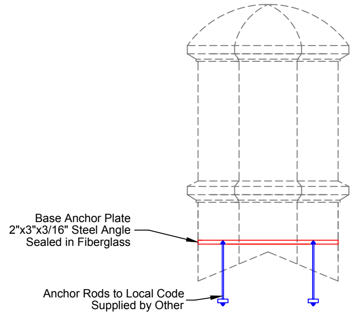
Skeleton View
