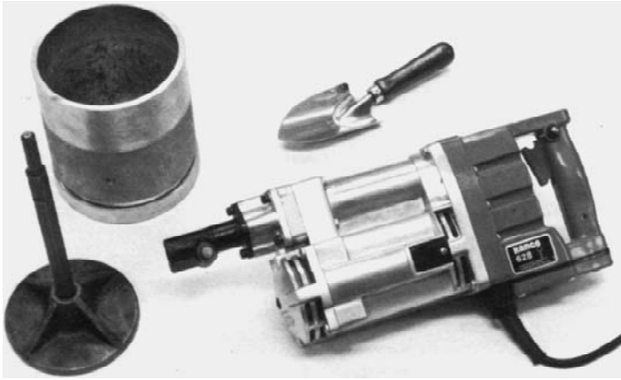
Figure 3.17 Electric vibrating hammer
