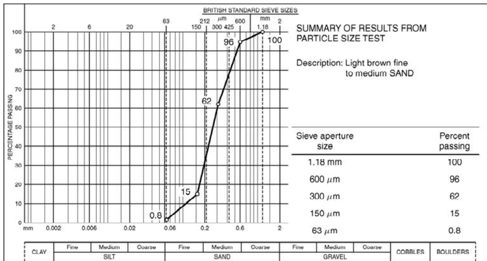
Figure 4.11 Results from particle size test and grading curve
