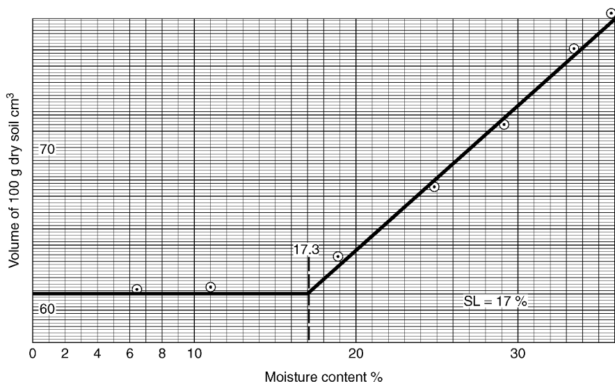
Figure 2.24 Shrinkage limit test results and graph (TRRL method)
