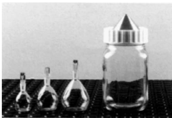
Figure 3.14 Density bottles and large pycnometer
