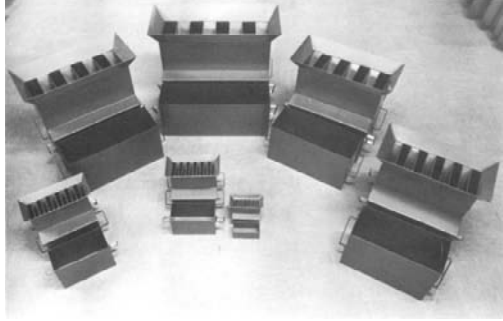
Figure 1.20 Riffle boxes
