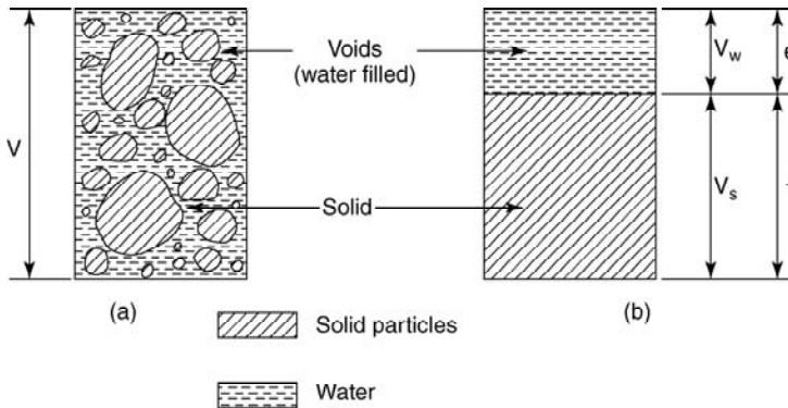
Figure 3.3 Representation of fully saturated soil
