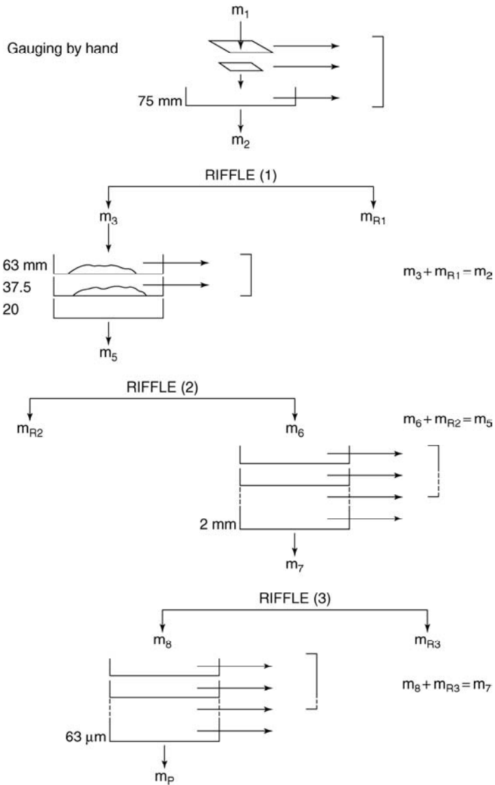
Figure 4.14 Sequence diagram, sieving with cobbles and boulders
