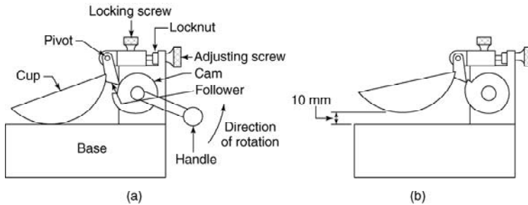
Figure 2.16 Principle of Casagrande apparatus
