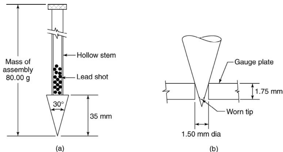
Figure 2.11 Details of cone for penetrometer
