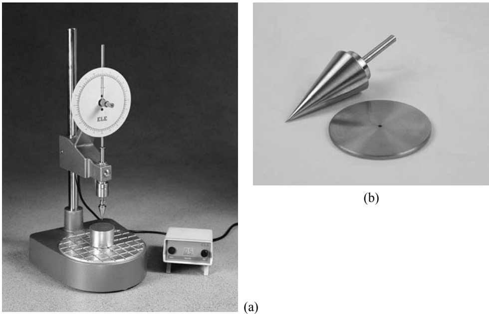
Figure 2.10 Apparatus for cone penetrometer liquid test: (a) Cone penetrometer with automatic timing device, (b) cone and gauge plate (photographs courtesy of ELE International)
