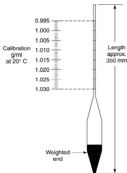
Figure 4.28 Soil hydrometer
