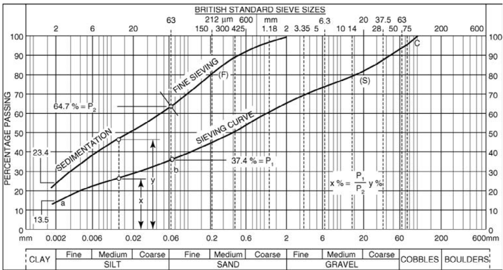
Figure 4.35 Combination of separate sieving and sedimentation curves ('boulder clay' type of soil)
