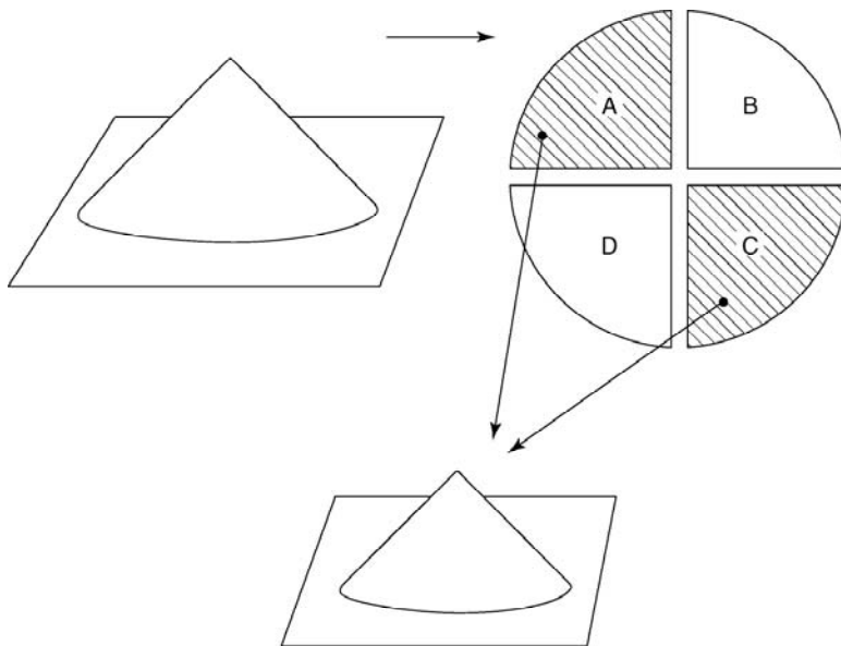
Figure 1.31 Cone-and-quartering
