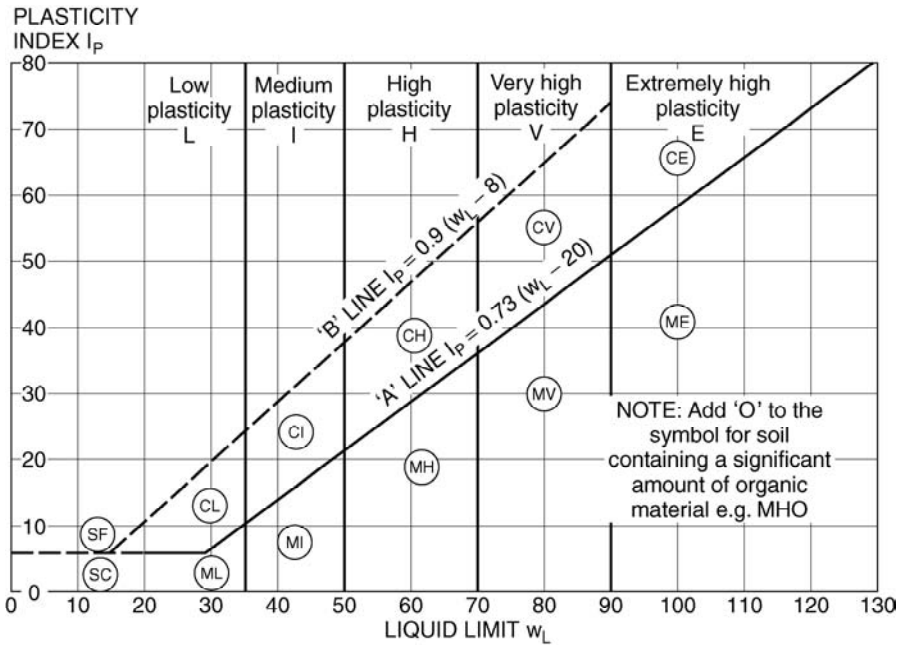
Figure 2.6 Plasticity chart
