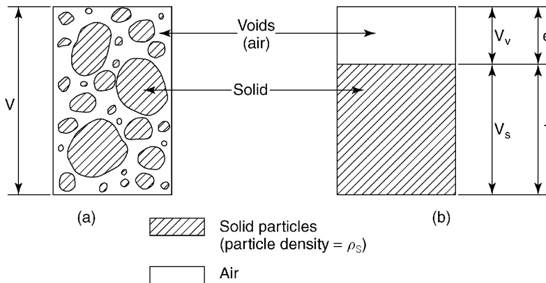
Figure 3.2 Representation of dry soil
