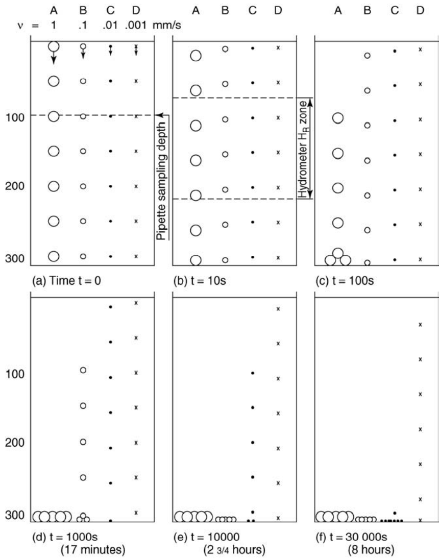
Figure 4.22 Representation of sedimentation process
