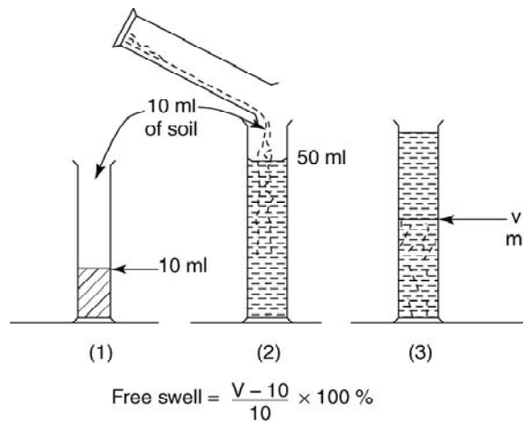
Figure 2.27 Free swell test
