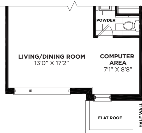
PARTIAL-SECOND FLOOR PLAN ELEVATION 'B'
