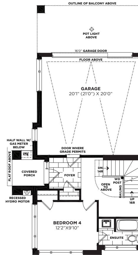
OPT. GROUND FLOOR PLAN 4 BEDROOM W/ BATH ELEVATION 'A'
