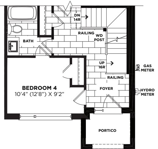
PARTIAL OPT GROUND FLOOR PLAN 4 BEDROOM W/ BATH ELEVATION 'B'
