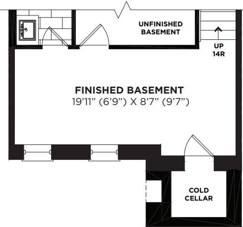
PARTIAL-BASEMENT FLOOR PLAN ELEVATION 'B'
