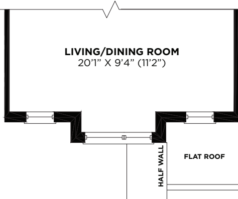
PARTIAL-SECOND FLOOR PLAN ELEVATION 'B'
