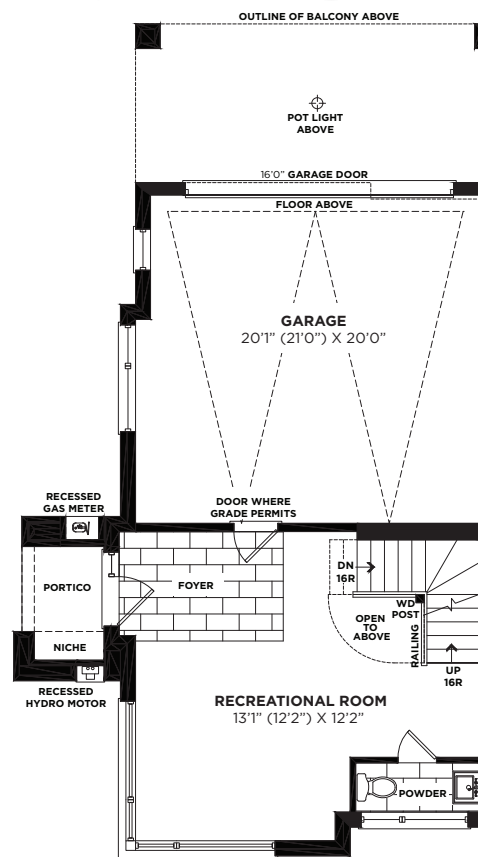
GROUND FLOOR PLAN ELEVATION 'B'
