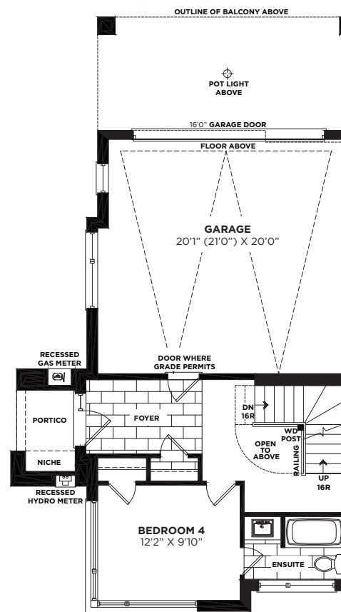
OPT. GROUND FLOOR PLAN BEDROOM W/ BATH ELEVATION 'B'
