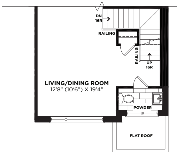
PARTIAL SECOND FLOOR PLAN ELEVATION 'B'
