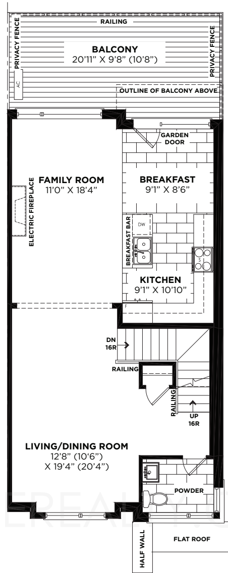
SECOND FLOOR PLAN ELEVATION 'A'
