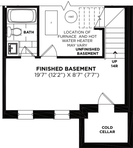
PARTIAL BASEMENT FLOOR PLAN ELEVATION 'B'
