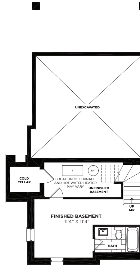
BASEMENT FLOOR PLAN ELEVATION 'A'
