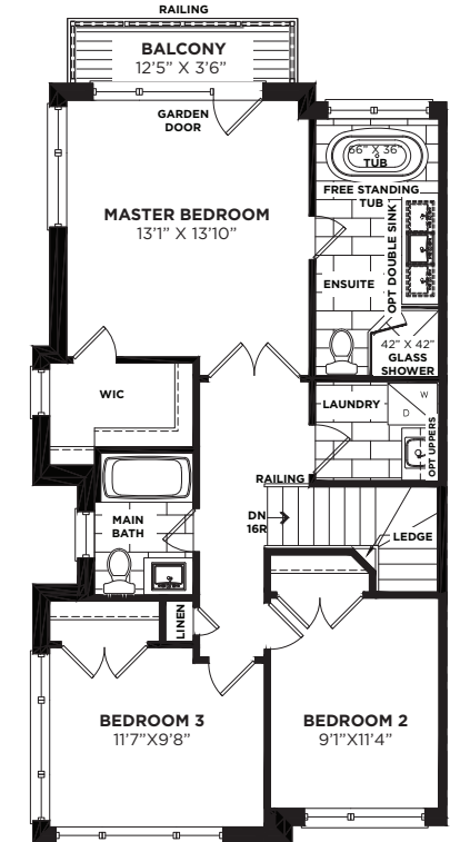
THIRD FLOOR PLAN ELEVATION 'A'
