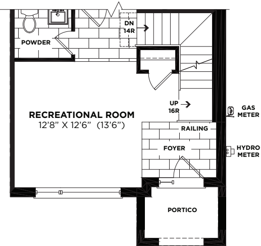
PARTIAL GROUND FLOOR PLAN ELEVATION 'B'
