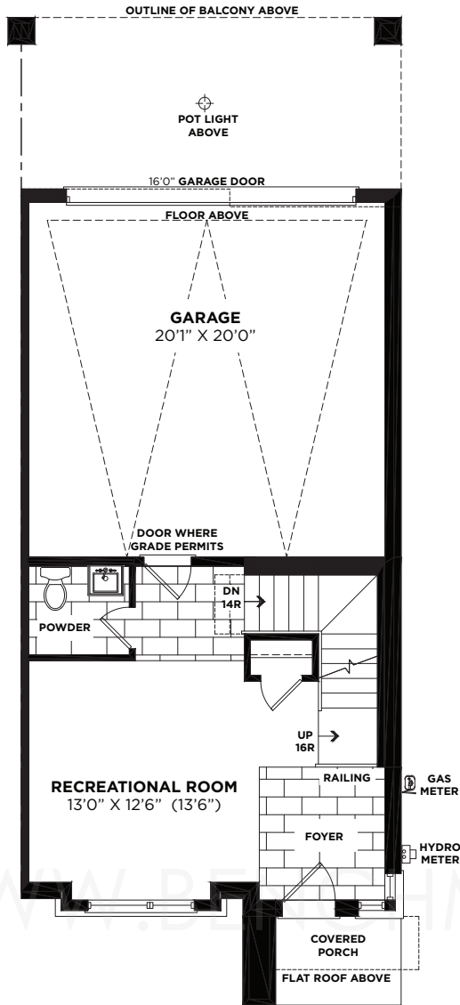
GROUND FLOOR PLAN ELEVATION 'A'
