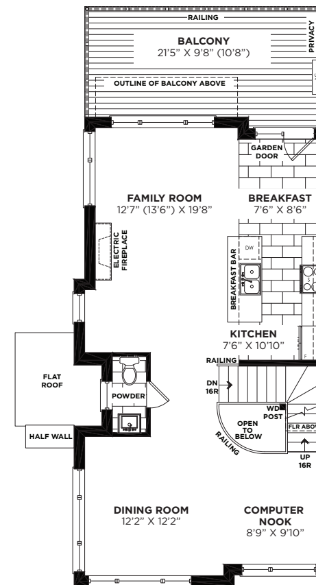
SECOND FLOOR PLAN ELEVATION 'A'
