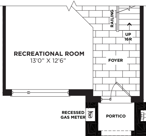
PARTIAL-GROUND FLOOR PLAN ELEVATION 'B'
