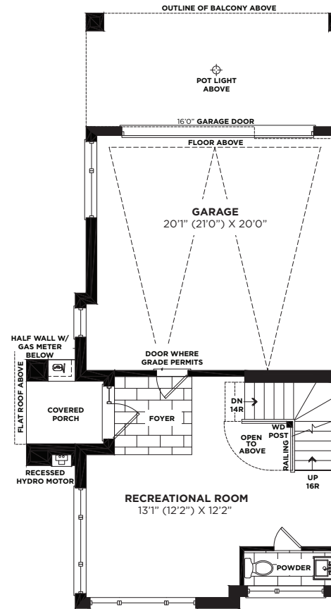
GROUND FLOOR PLAN ELEVATION 'A'
