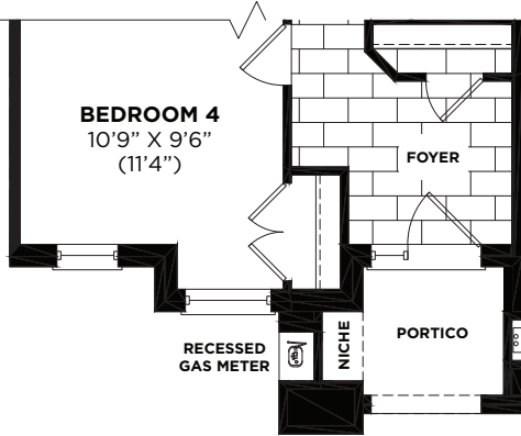
PARTIAL-OPT. GROUND FLOOR PLAN 4 BEDROOM W/ BATH ELEVATION 'B'
