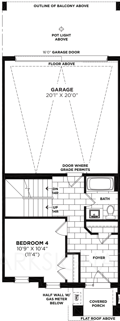
OPT. GROUND FLOOR PLAN 4 BEDROOM W/ BATH ELEVATION 'A'
