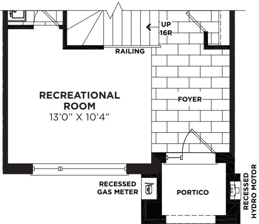
PARTIAL-GROUND FLOOR PLAN ELEVATION 'B'
