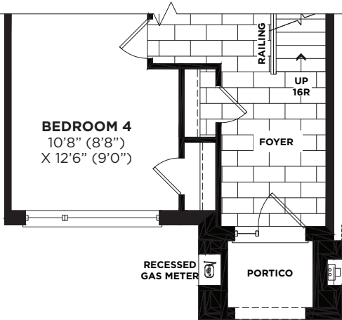
PARTIAL-OPT. GROUND FLOOR PLAN BEDROOM W/ BATH ELEVATION 'B'
