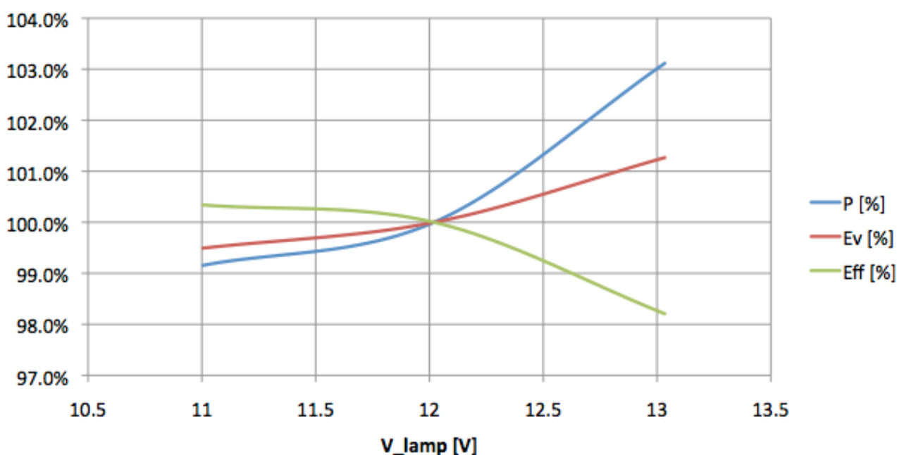
Dependency on lamp parameters on V_{\text{lamp}}
