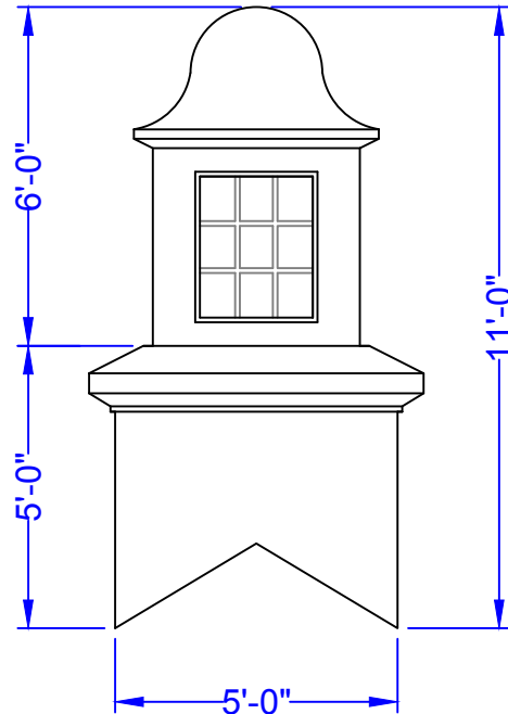
Elevation View
