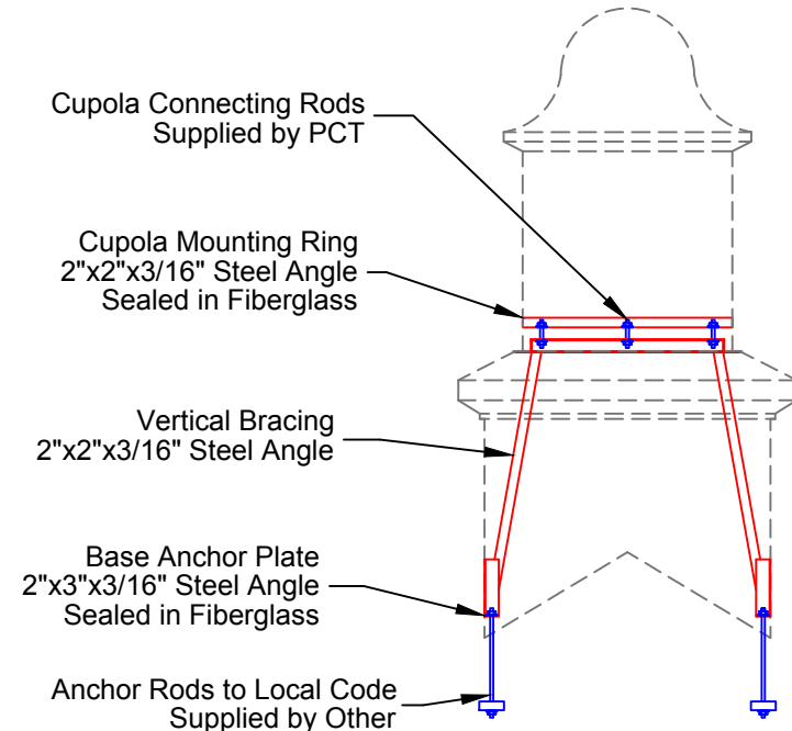
Skeleton View
