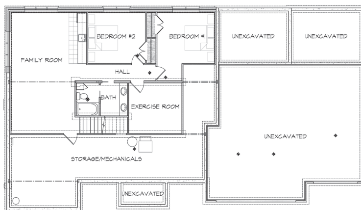
FOUNDATION PLAN
