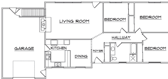
PRE-ADDITION LAYOUT
