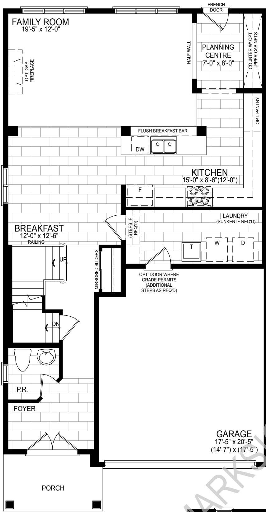
GROUND FLOOR PLAN STYLE A
