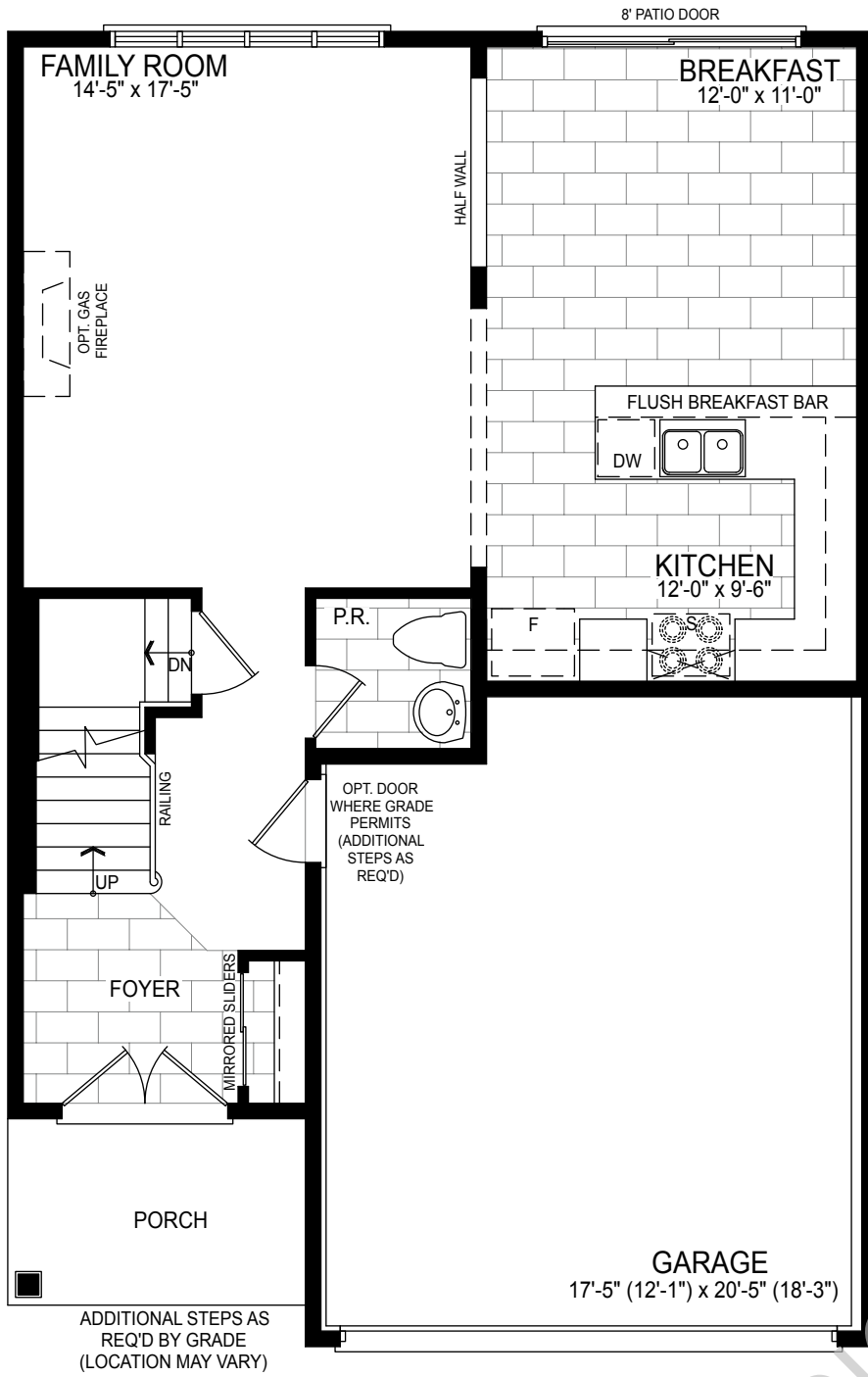
GROUND FLOOR PLAN STYLE A
