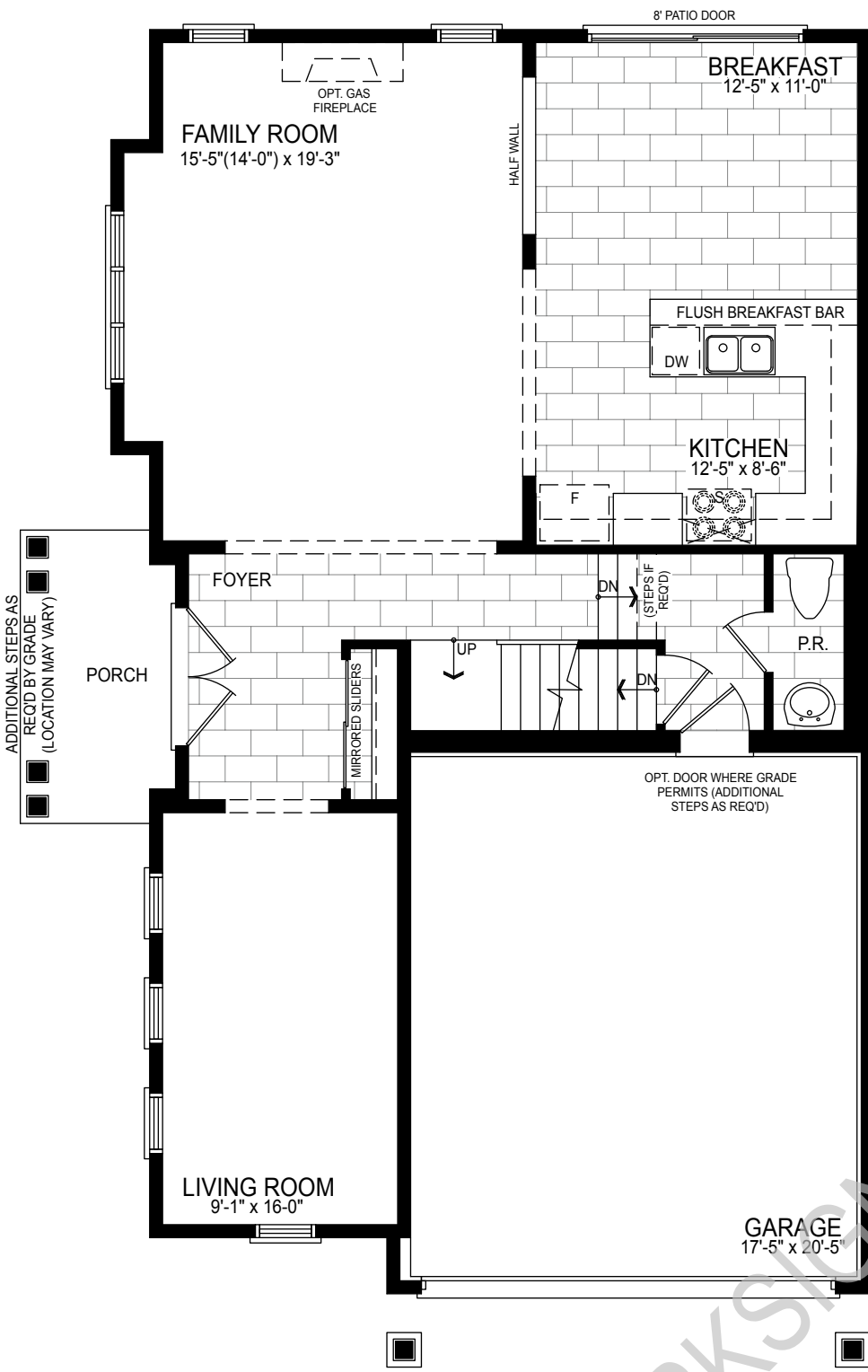
GROUND FLOOR PLAN STYLE A
