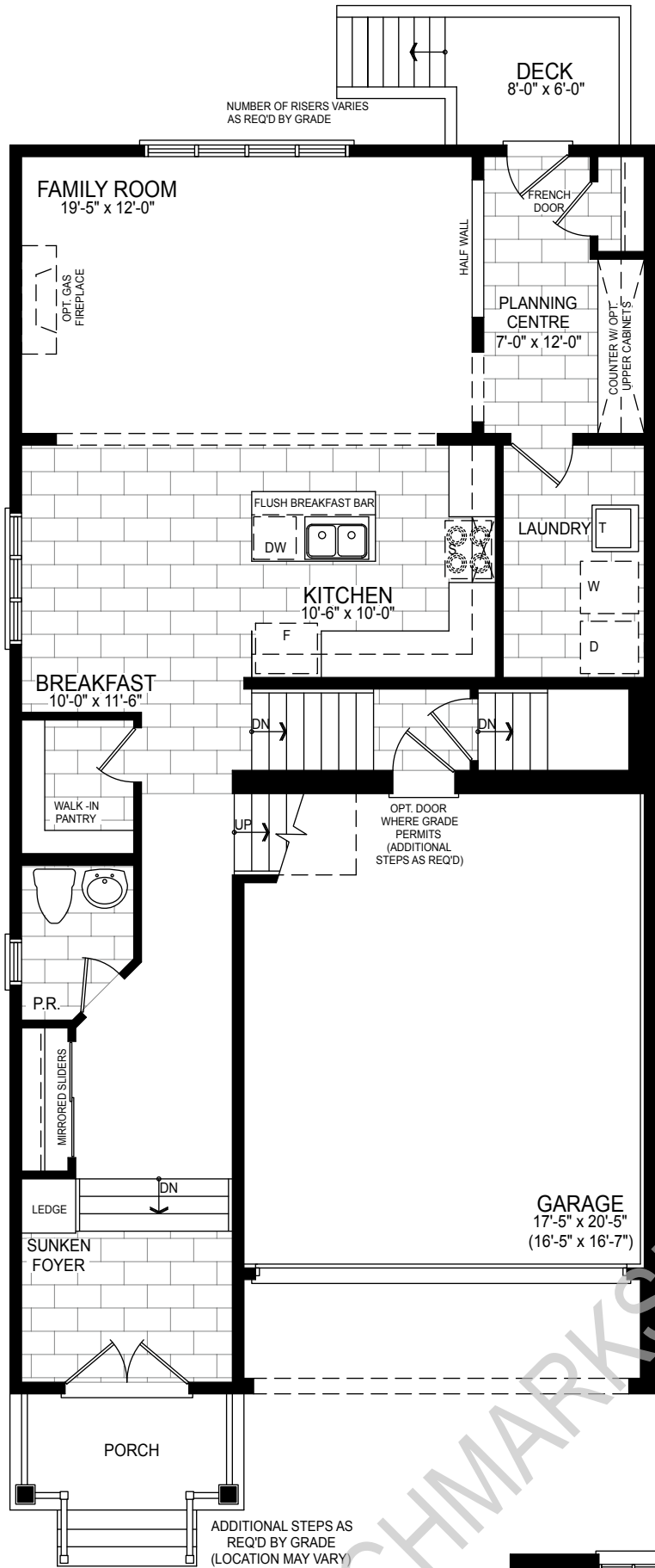
GROUND FLOOR PLAN STYLE A
