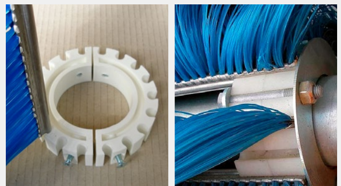
Holding device for the strip brushes
