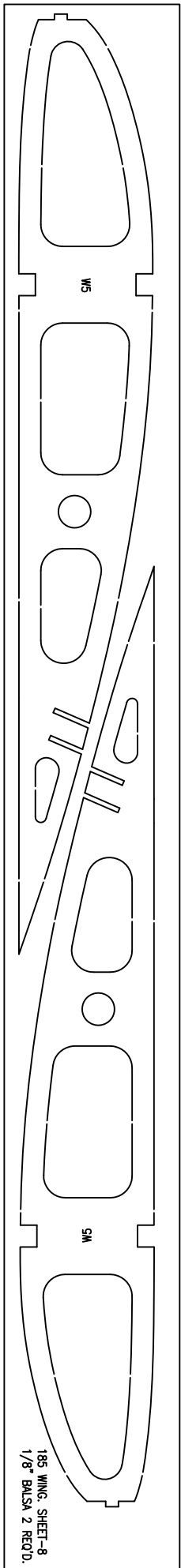
4" WIDE x 36" LONG x 1/8" THICK BALSA TWO (2) REQUIRED
