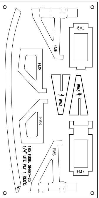
6" WIDE x 12" LONG x 1/4" THICK Lite Ply ONE (1) REQUIRED
