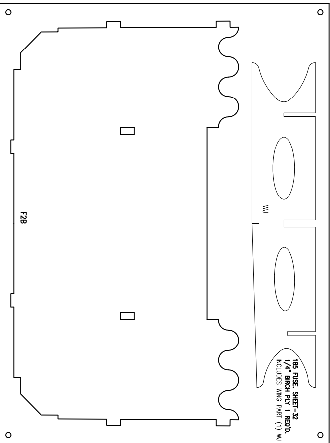
12" WIDE x 16" LONG x 1/4" THICK BIRCH PLY ONE (1) REQUIRED
