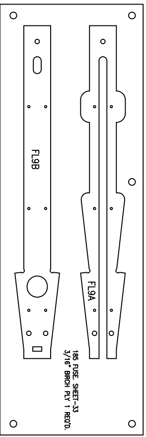
4" WIDE x 12" LONG x 3/16" THICK BIRCH PLY ONE (1) REQUIRED
