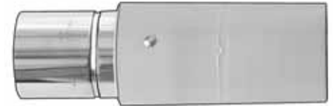
Hose cuff reducer 1.25" dia. hose with 1.5" dia steel tube Part # 1B52025
