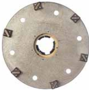
Magpie Aluminum cutting head c/w 6 Gimlet 16 grit diamonds Part # 2A81840
