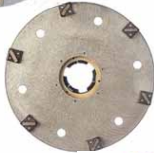
Magpie Aluminum cutting head c/w 6 Gimlet 16 grit diamonds Part # 2A81836
