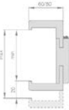
RANGE OF ADJUSTABLE DOOR FRAME above 280 mm
