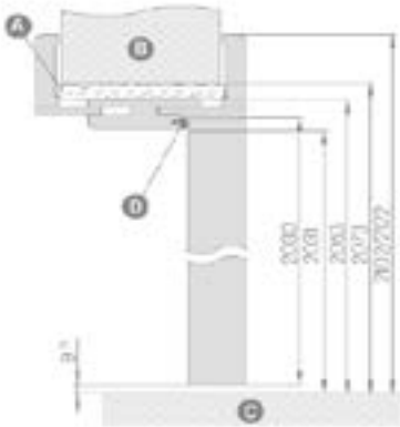
HEIGHT IN PL* STANDARD
