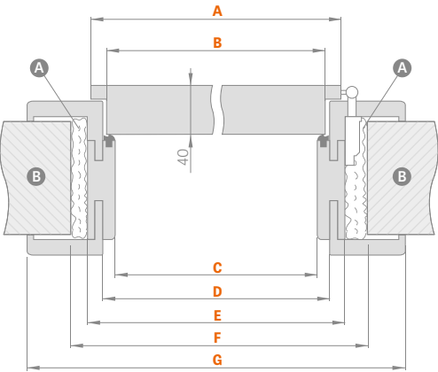
DIAGRAM OF ADJUSTABLE DOOR FRAME strip 6 cm / strip 8 cm
