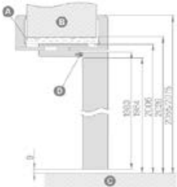
HEIGHT IN CZ* STANDARD (-47mm)
