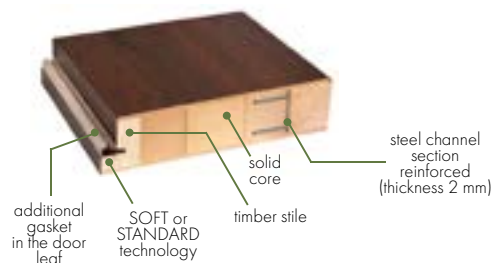
CROSS-SECTION OF HERSE DOOR LEAF 32 dB
