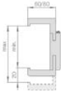
Adjustable door frame range
