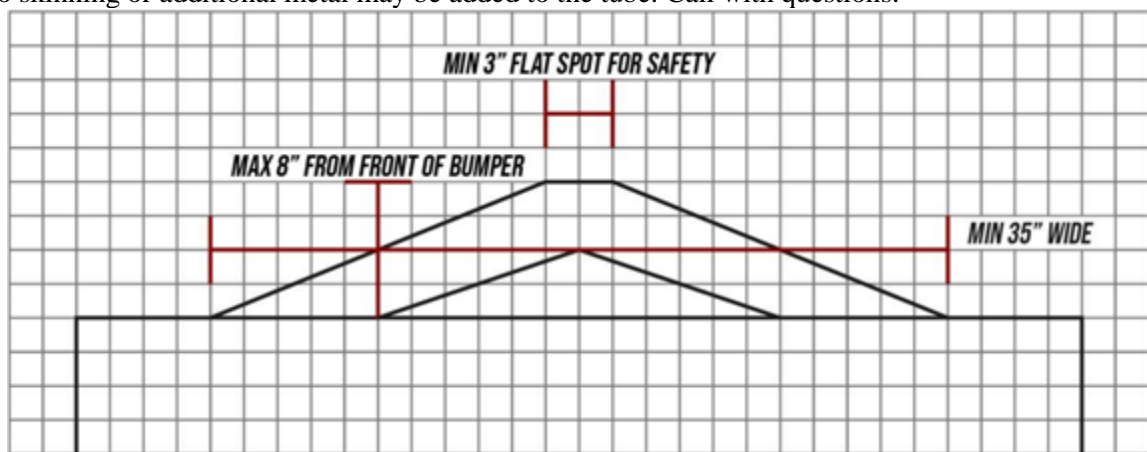
Bumper Diagram
