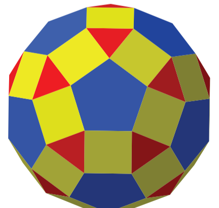
Rhombicosidodecahedron
