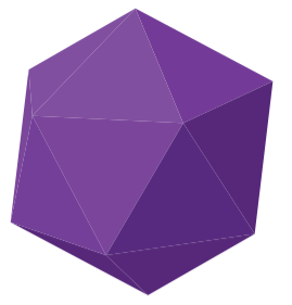
Icosahedron
