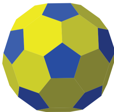
Truncated icosahedron
