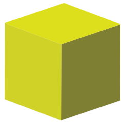
Cube (Hexahedron)
