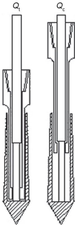
Figure 2 — M1 cone penetrometer (mantle)
