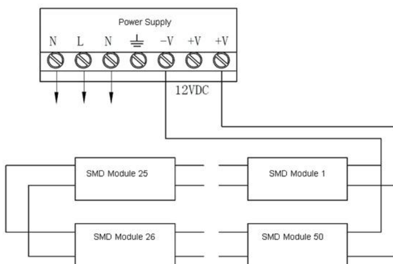
Connecting Diagram
