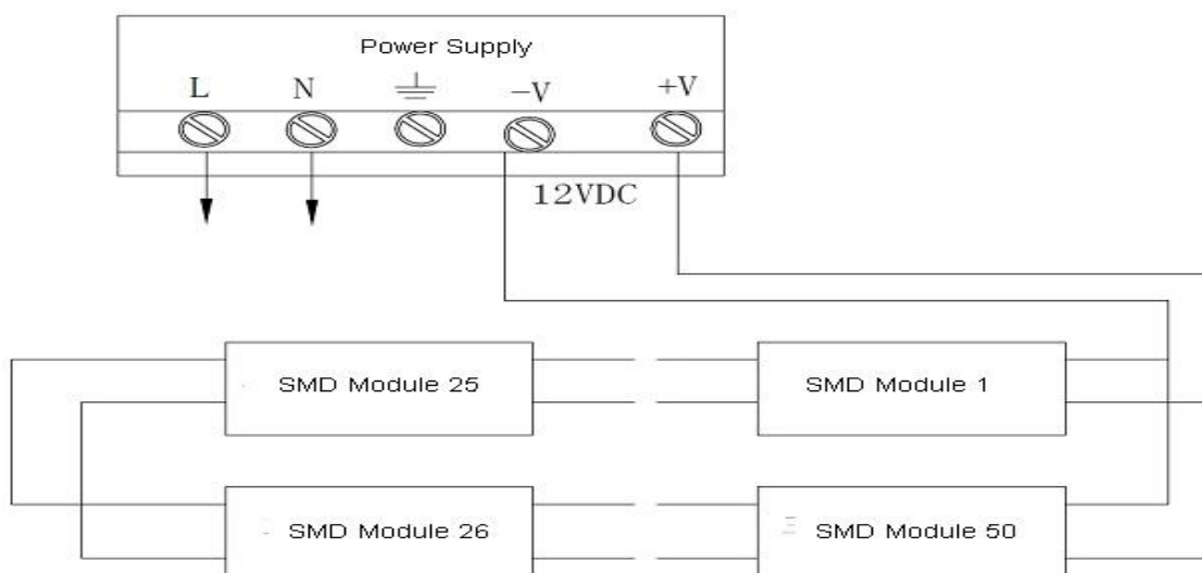
Connecting Diagram
