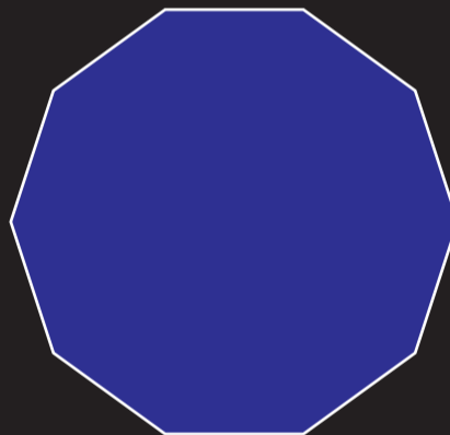
Decagon
