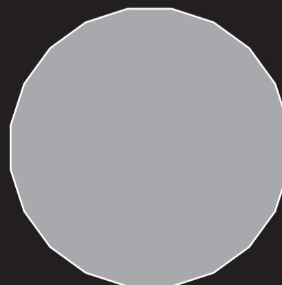
Icosagon
