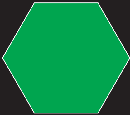
Hexagon
