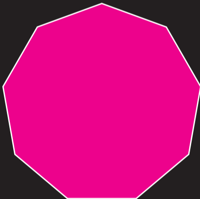
Nonagon
