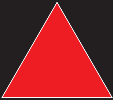
Triangle
