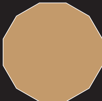
Dodecagon
