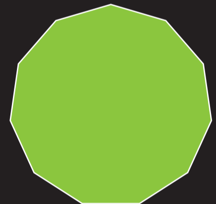
Undecagon
