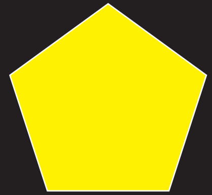
Pentagon
