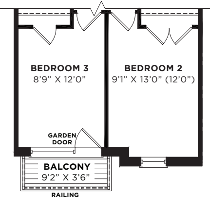
PARTIAL - THIRD FLOOR PLAN ELEVATION 'B'
