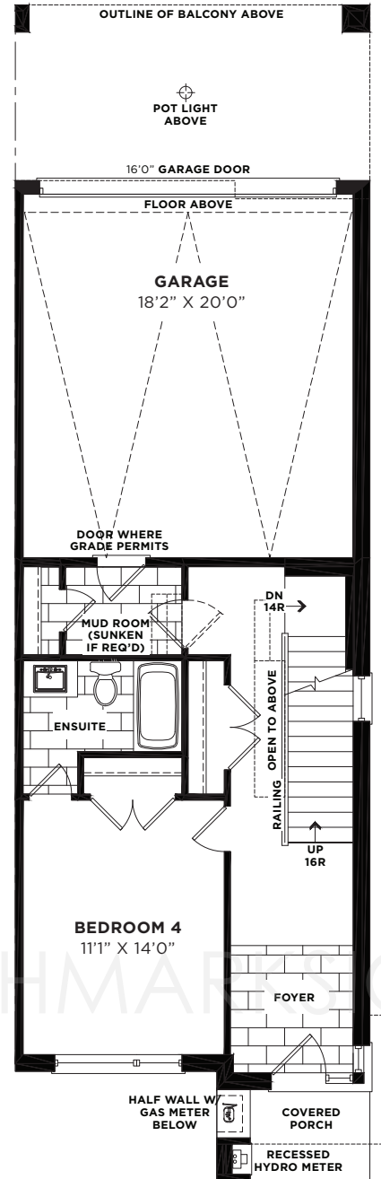
OPT. GROUND FLOOR PLAN 4 BEDROOM W/ ENSUITE ELEVATION 'A'
