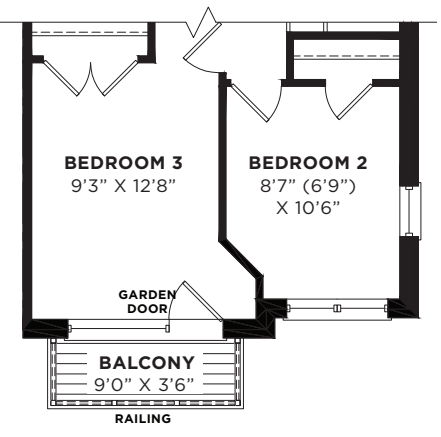
PARTIAL - THIRD FLOOR PLAN ELEVATION 'B'
