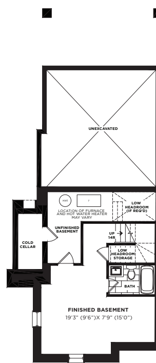
PARTIAL - BASEMENT FLOOR PLAN ELEVATION 'B'
