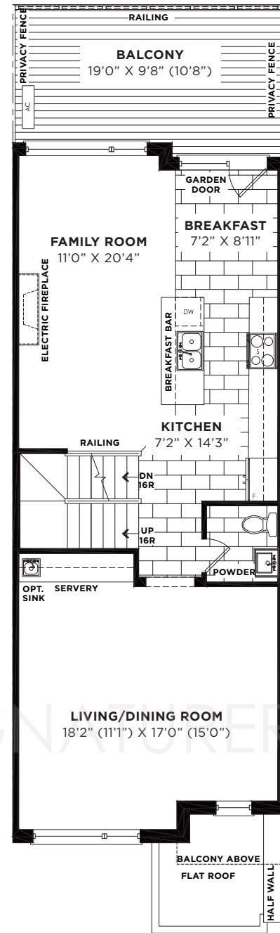
SECOND FLOOR PLAN ELEVATION 'A'
