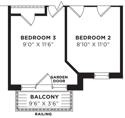
PARTIAL - THIRD FLOOR PLAN ELEVATION 'B'
