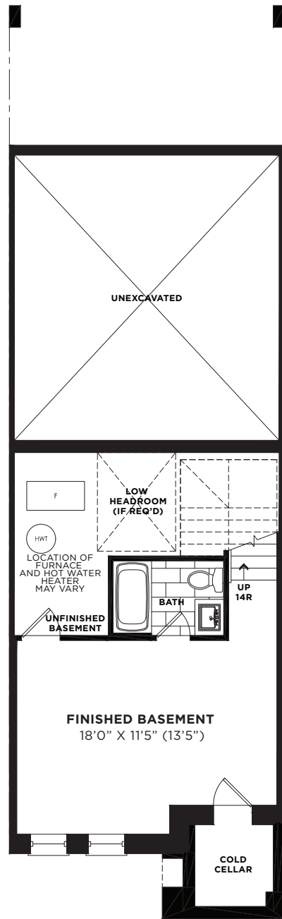
BASEMENT FLOOR PLAN ELEVATION 'A'
