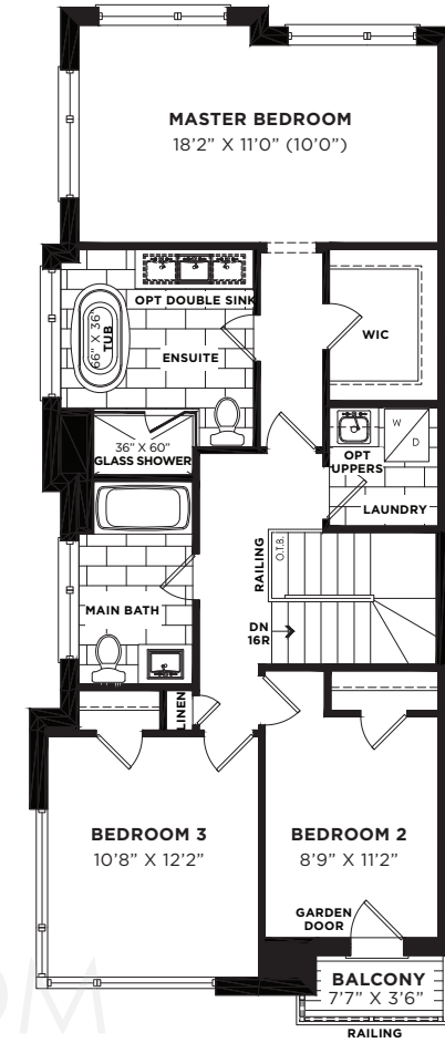
THIRD FLOOR PLAN ELEVATION 'A'
