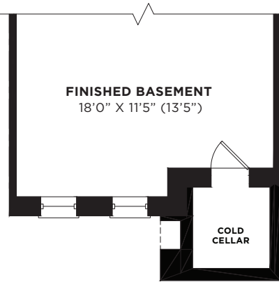
PARTIAL - BASEMENT FLOOR PLAN ELEVATION 'B'
