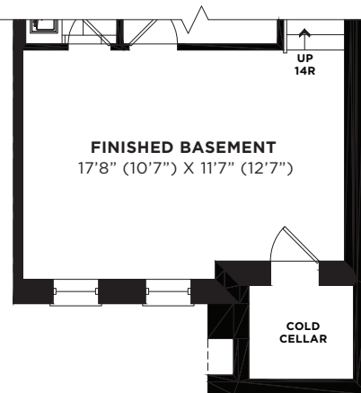
PARTIAL - BASEMENT FLOOR PLAN ELEVATION 'B'
