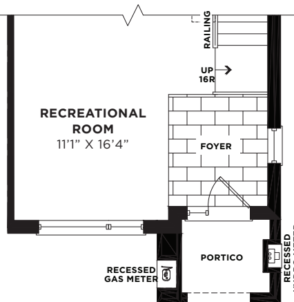
PARTIAL - GROUND FLOOR PLAN ELEVATION 'B'
