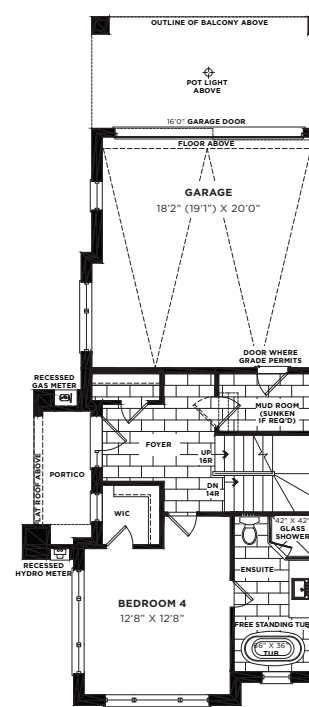
PARTIAL - OPT. GROUND FLOOR PLAN 4 BEDROOM W/ ENSUITE ELEVATION 'B'
