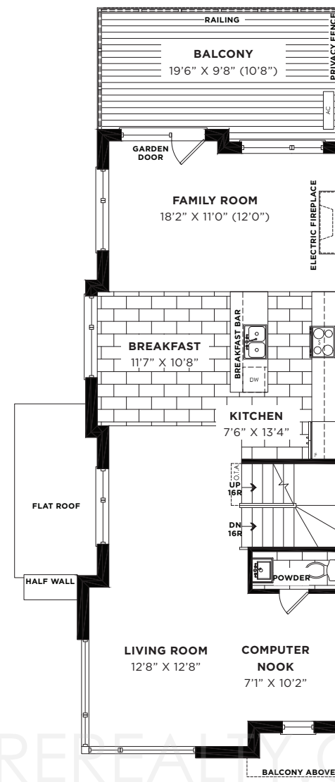
SECOND FLOOR PLAN ELEVATION 'A'
