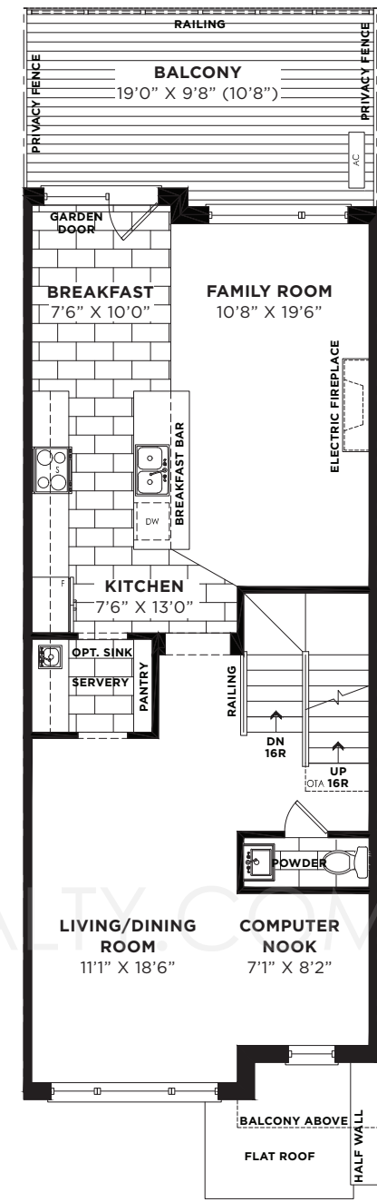
OPT. SECOND FLOOR PLAN ELEVATION 'A'
