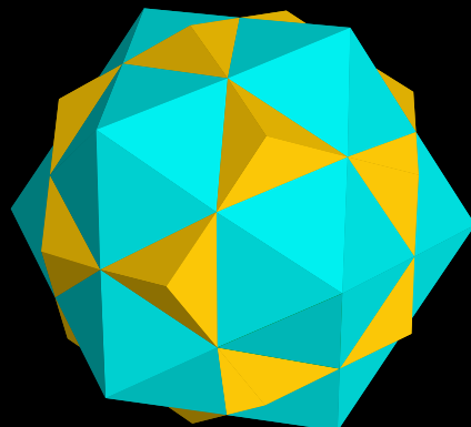
Dodecahedron and Icosahedron
