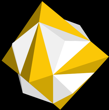
Dodecahedron and Octahedron
