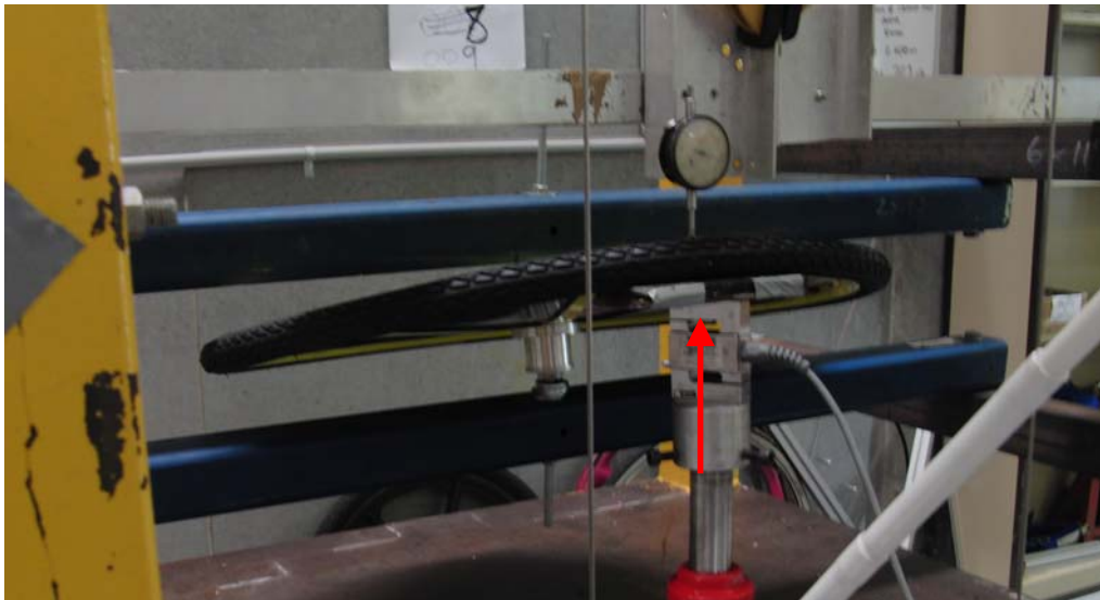
Figure 2: Deflection reached at maximum applied load in Test 1.
