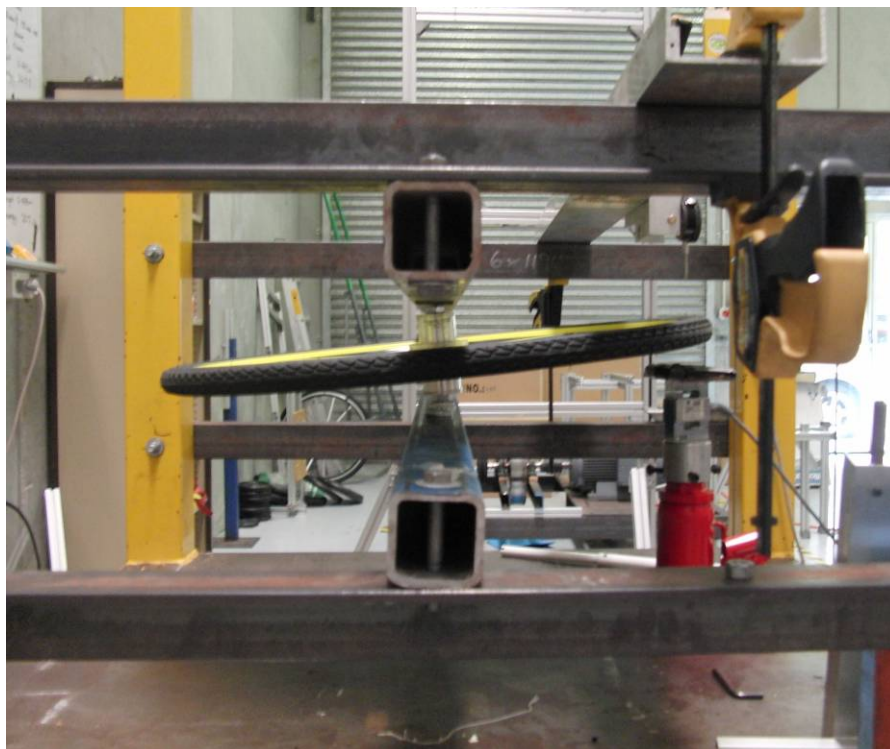
Figure 3: Residual deflection of wheel following removal from test rig
