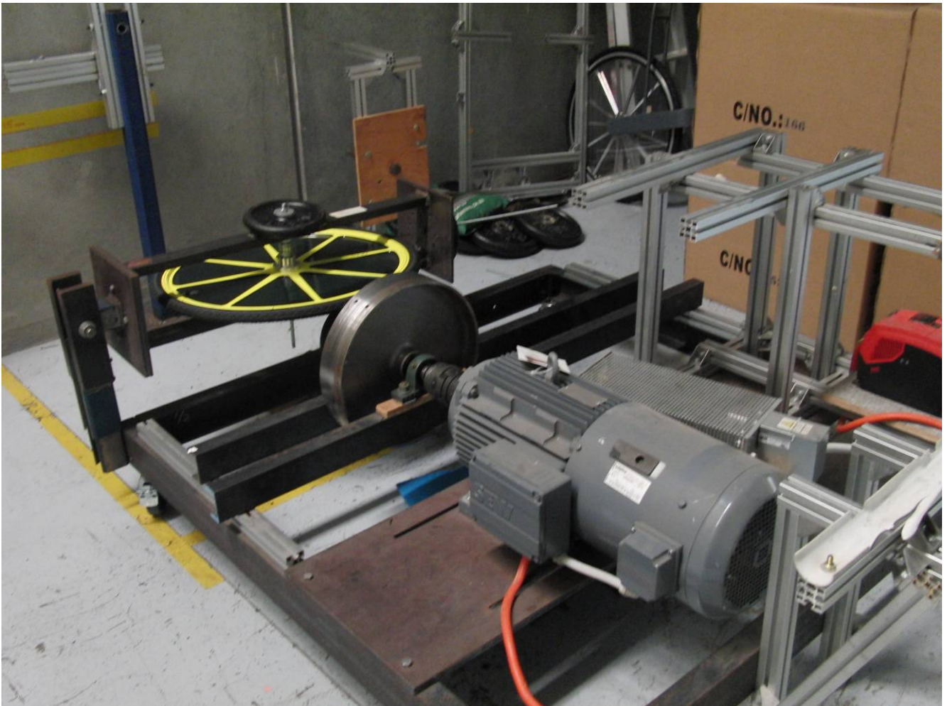
Figure 4 Fatigue test
