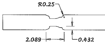
Standard Sticking / Beaded Panel
