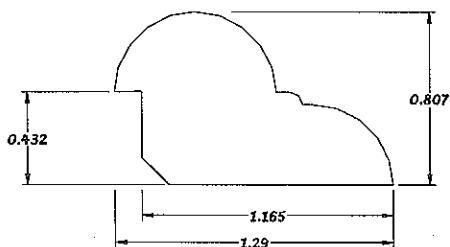
ERM 01 Profile
