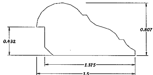
ERM 02 Profile
