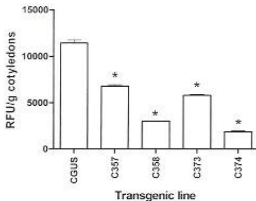
Figure 6 Growth of Aspergillus flavus 70-GFP on cotyledons of immature T1 cotton seed 7 days after inoculation as measured by the fluorescence emanating from the fungus. (*) denotes a significant reduction ( P < 0.05 ) in the fluorescence in seed cotyledons of transgenic lines compared to that of CGUS negative control seed cotyledons. Error bars indicate standard error of means. Mean separation was performed using the method of Tukey following ANOVA.
