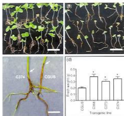
Figure 8 Antifungal assay in planta with T1 progeny seedlings of transgenic cotton plants expressing the synthetic peptide D4E1 against a seedling pathogen, Thielaviopsis basicola . (a) Seedlings of C374 showing healthy root system and increased vigor. (b) Seedlings of CGUS negative controls – note the reduction in vigor and black discoloration on hypocotyls and roots with reduced or no branching in CGUS negative control seedlings. (c) A close-up of the typical black root rot lesions caused by T. basicola , on cotton seedling hypocotyls (arrows) of C374 and CGUS negative control two weeks after planting in soil inoculated with the fungus. Note lack of root branching on discolored primary root of controls compared to C374. (d) Fresh weight of seedlings ( n = c. 150 ) grown for two weeks on inoculated soil with T. basicola . Transgenic cotton line C357 was not included in this assay. Note significant ( P < 0.05 ) increase in fresh weight of seedlings from D4E1 -transgenic lines compared to CGUS negative controls. Scale bars indicate 60 mm in a, and b; 15 mm in c.
