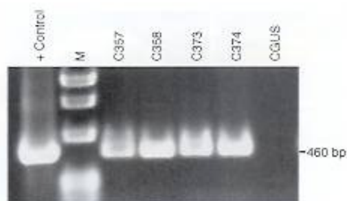
Figure 2 PCR of transgenic cotton genomic DNA – total DNA from transgenic cotton was amplified with primers designed to an approximate 460-bp region spanning from within the d35S promoter to the 3' end of the nos terminator. Lane CGUS represents PCR amplification using pBI-d35S \Omega -uidA-nos genomic template DNA (negative control). Lane 'M' represents Hae III digested phi X-174 marker DNA; + control denotes pBI-d35S \Omega -D4E1-nos plasmid DNA-positive control.
