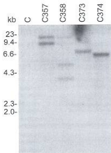
Figure 1 Southern hybridization of d35SΩ-D4E1 transgenic T1 cotton genomic DNA – Southern hybridization of genomic DNA of four cotton T1 plants transformed with pBI-d35SΩ-D4E1-nos and a non-transformed cotton plant (Lane C) was performed to demonstrate the successful integration of the transgene. The membrane was probed with a radiolabelled HindIII - SacI fragment representing the d35SΩ-D4E1 region of approximately 900 bp.
