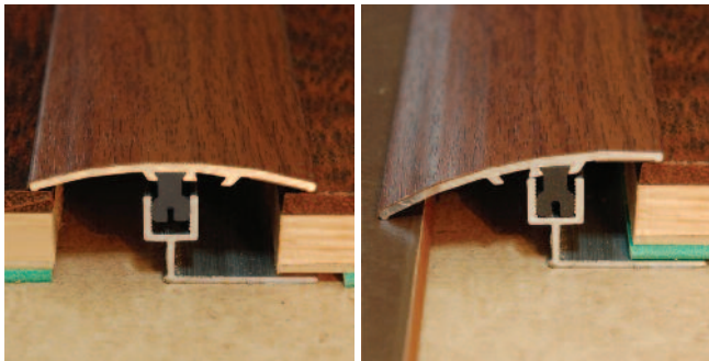
Prestige Universal Connector for surfaces of even height or small ramp for surfaces of uneven heights
