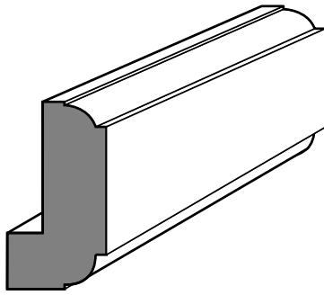
1 1/8" Panel Cap
