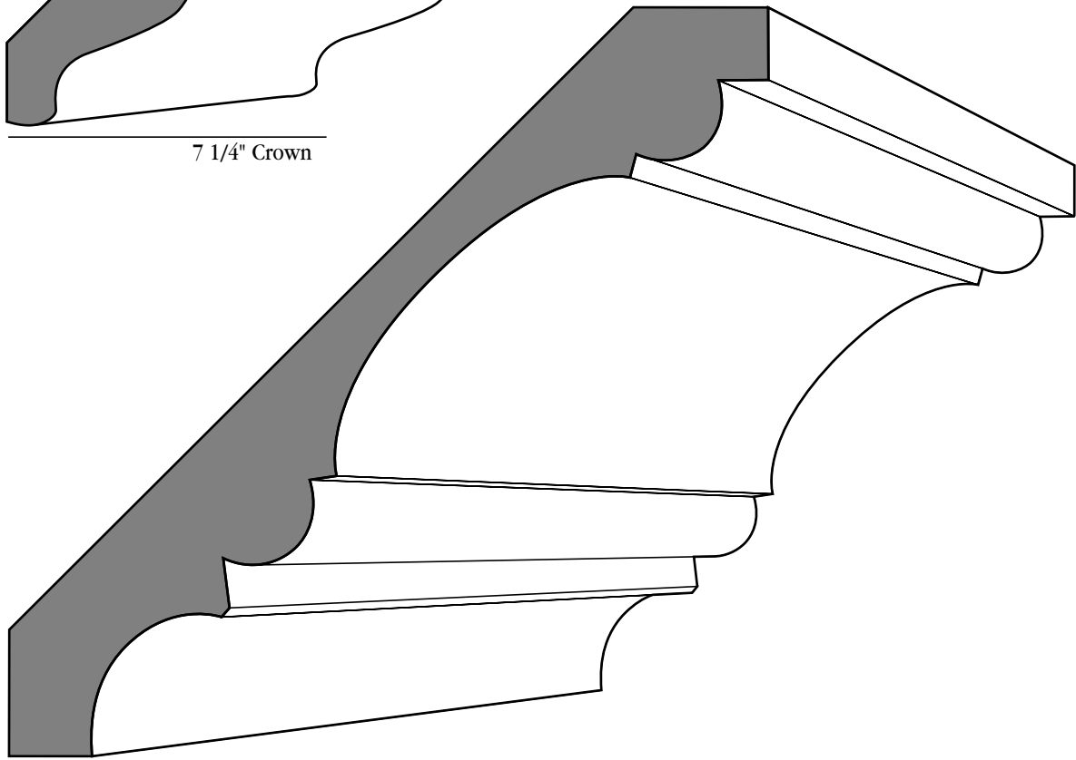
6" Themis Crown
