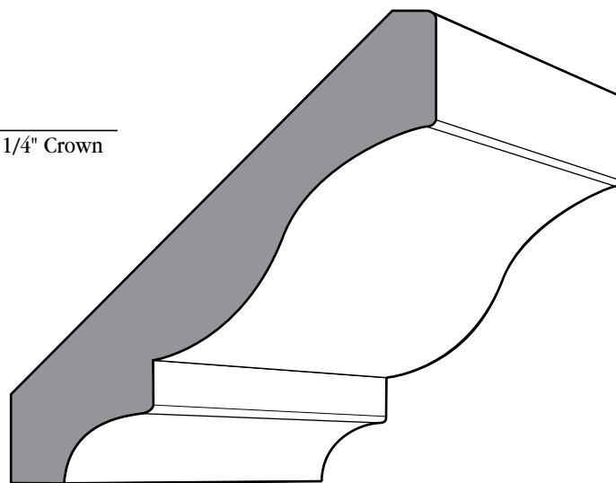
3 5/8" Crown
