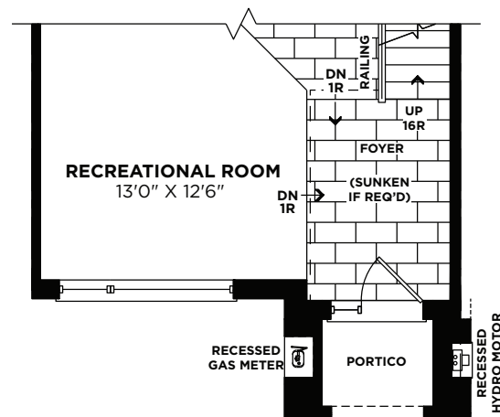
PARTIAL GROUND FLOOR PLAN ELEVATION 'B'
