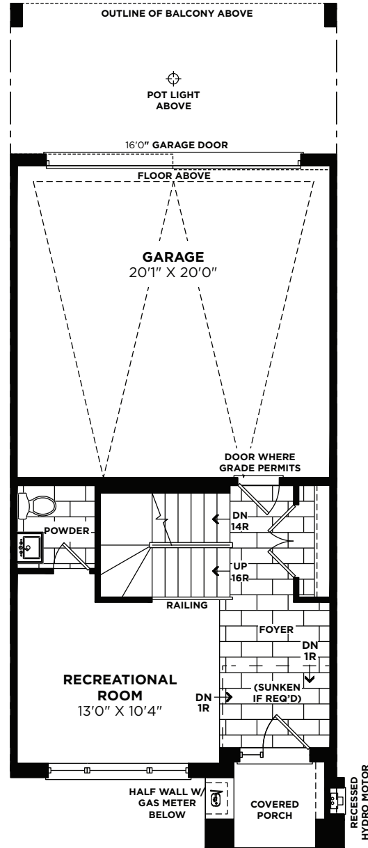
GROUND FLOOR PLAN ELEVATION 'A'
