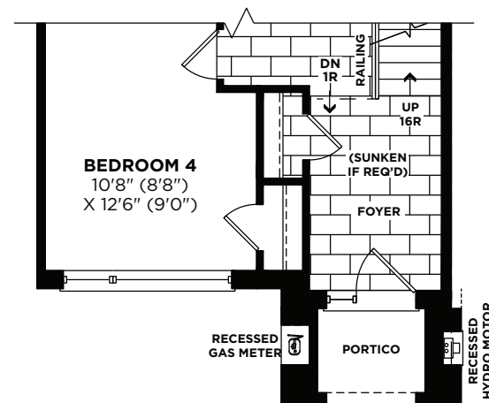
PARTIAL OPT. GROUND FLOOR PLAN BEDROOM W/ BATH ELEVATION 'B'
