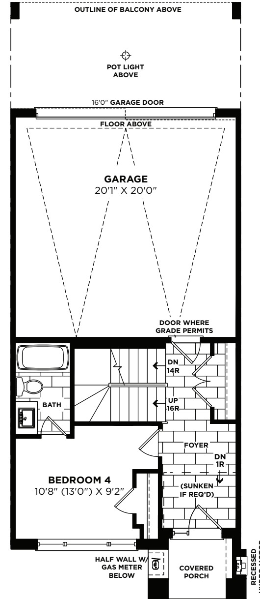
OPT. GROUND FLOOR PLAN 4 BEDROOM W/ BATH ELEVATION 'A'
