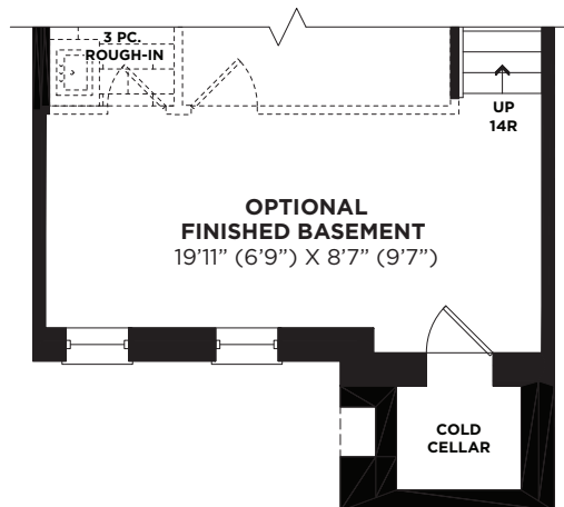
PARTIAL BASEMENT FLOOR PLAN ELEVATION 'B'
