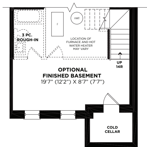
PARTIAL BASEMENT FLOOR PLAN ELEVATION 'B'
