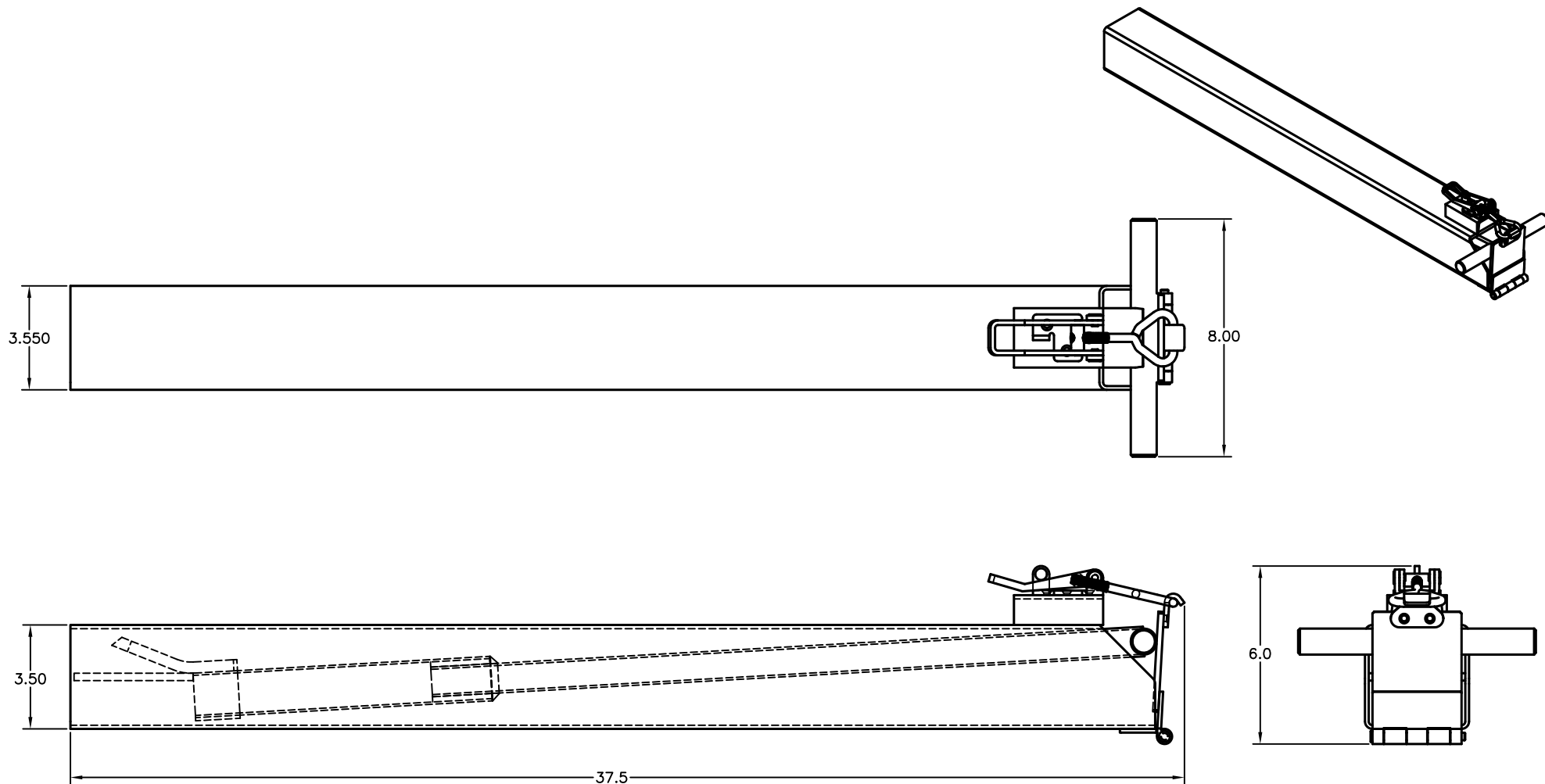
BOOM DOG OUTLINE DIMENSIONS
