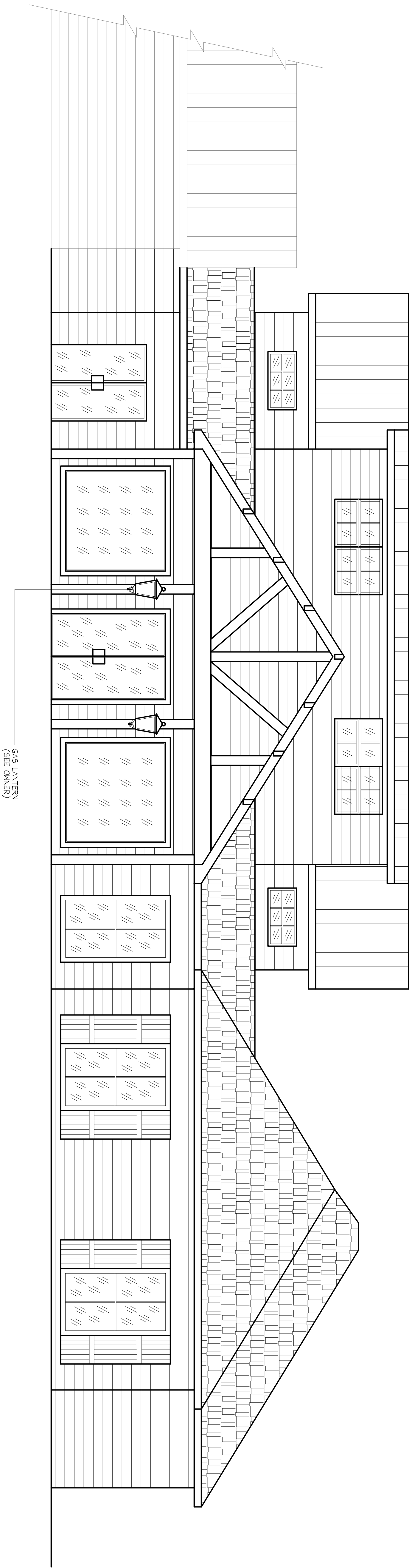
PROPOSED EXTERIOR ELEVATION SCALE 1/4" = 1'-0"
