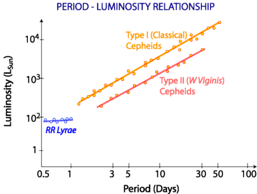
Period-luminosity relationship for Cepheids and RR Lyrae stars.
