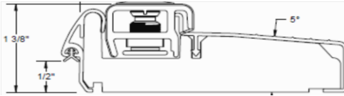
All Aluminum Tile Back 3-11/16" & 4-9/16"
